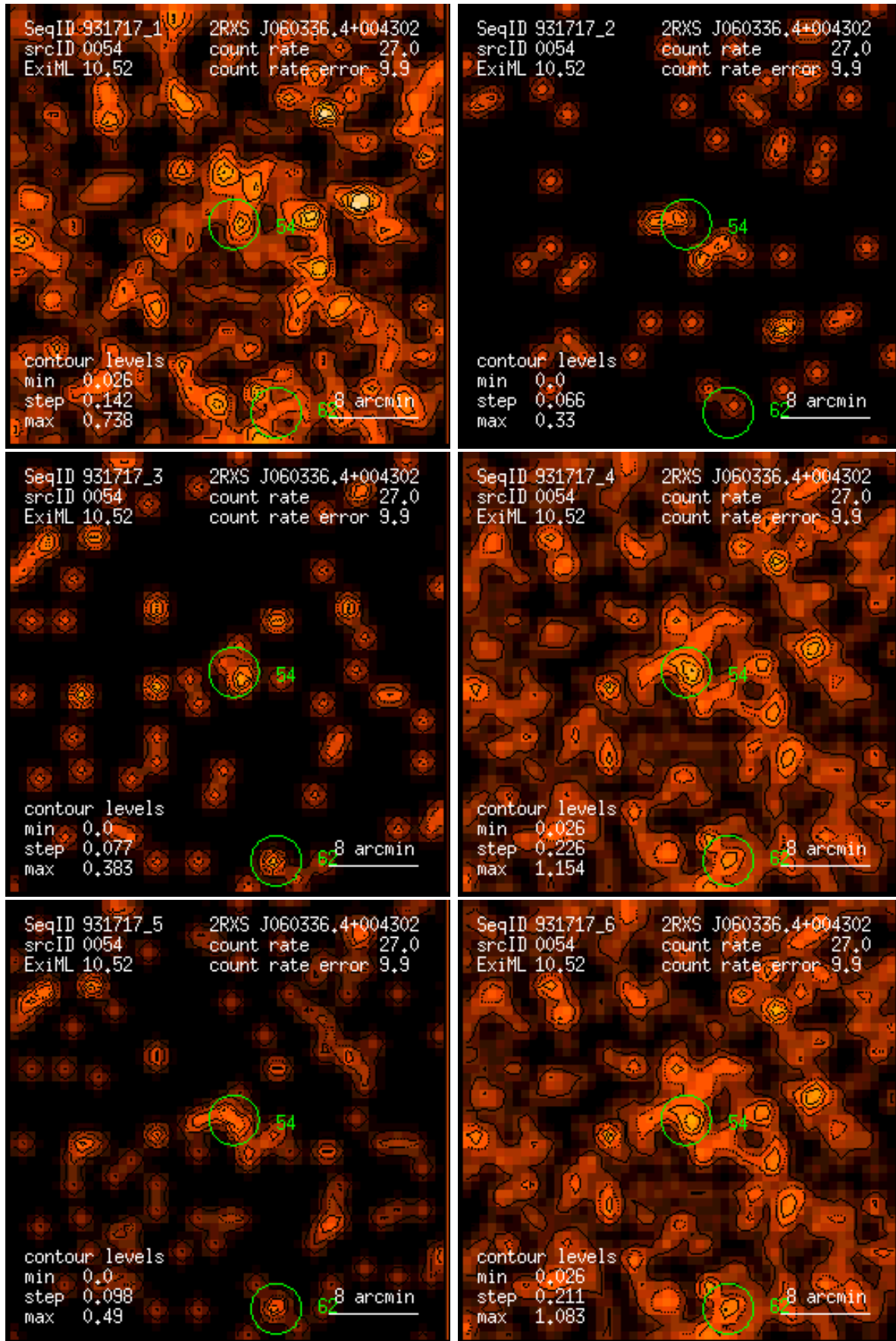
Figure 54: RASS 931717: detection 0054: band rate images, Gaussian filter: (1) PSPC channels 11 – 41, (2) 52 – 90, (3) 91 – 201, (4) 11 – 235, (5) 52 – 201, (6) 11 – 201. Broad band rates in counts/ks. Band rate contour levels in counts/ks/arcmin 2 .
