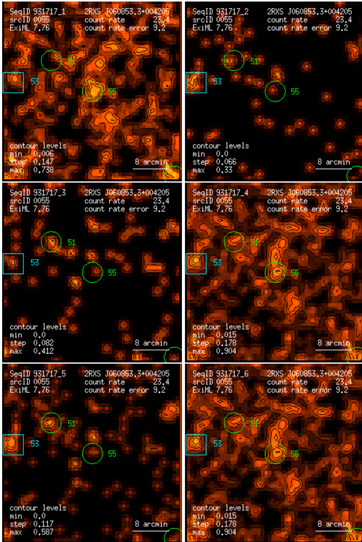
Figure 55: RASS 931717: detection 0055: band rate images, Gaussian filter: (1) PSPC channels 11 – 41, (2) 52 – 90, (3) 91 – 201, (4) 11 – 235, (5) 52 – 201, (6) 11 – 201. Broad band rates in counts/ks. Band rate contour levels in counts/ks/arcmin 2 .
