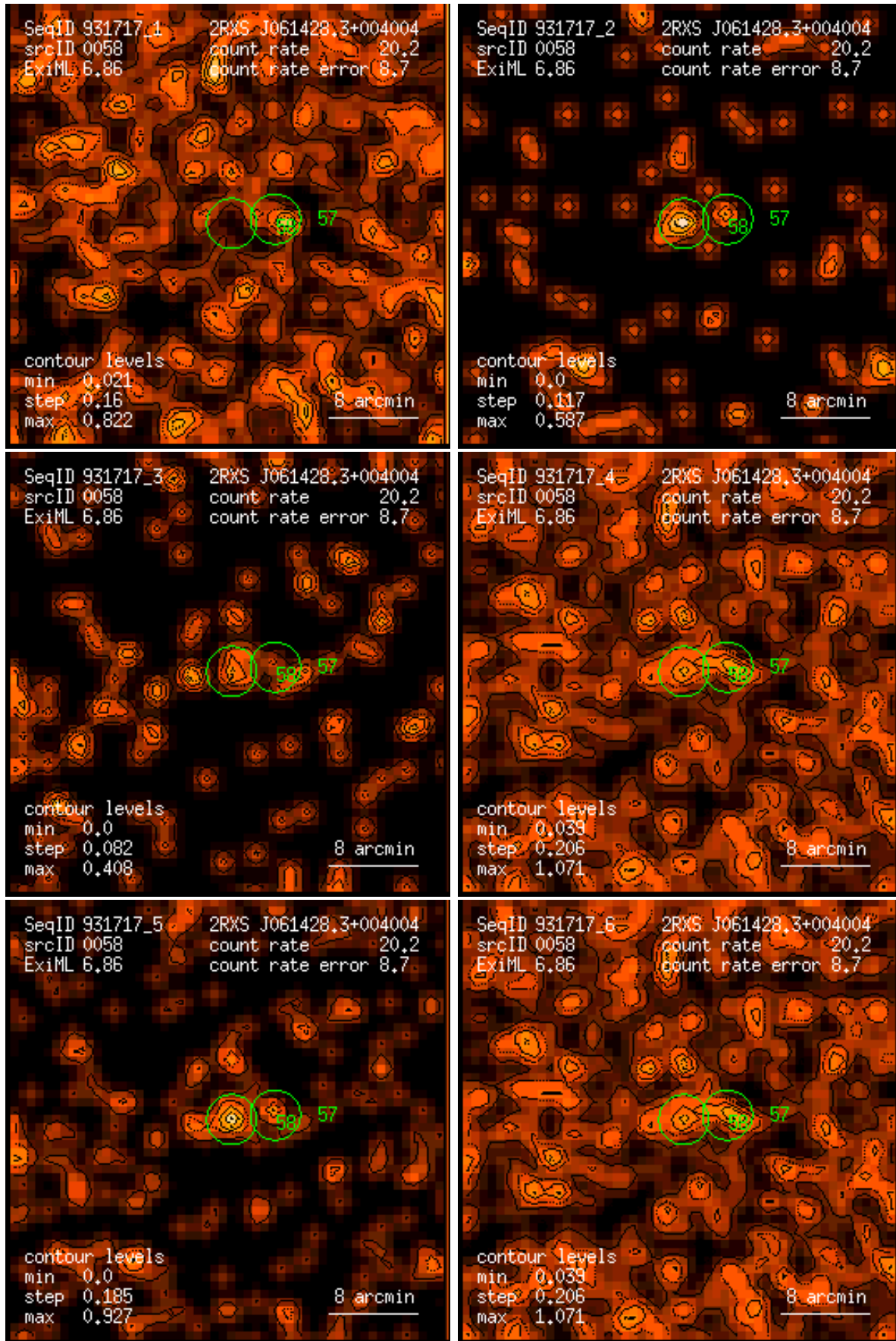
Figure 58: RASS 931717: detection 0058: band rate images, Gaussian filter: (1) PSPC channels 11 – 41, (2) 52 – 90, (3) 91 – 201, (4) 11 – 235, (5) 52 – 201, (6) 11 – 201. Broad band rates in counts/ks. Band rate contour levels in counts/ks/arcmin 2 .
