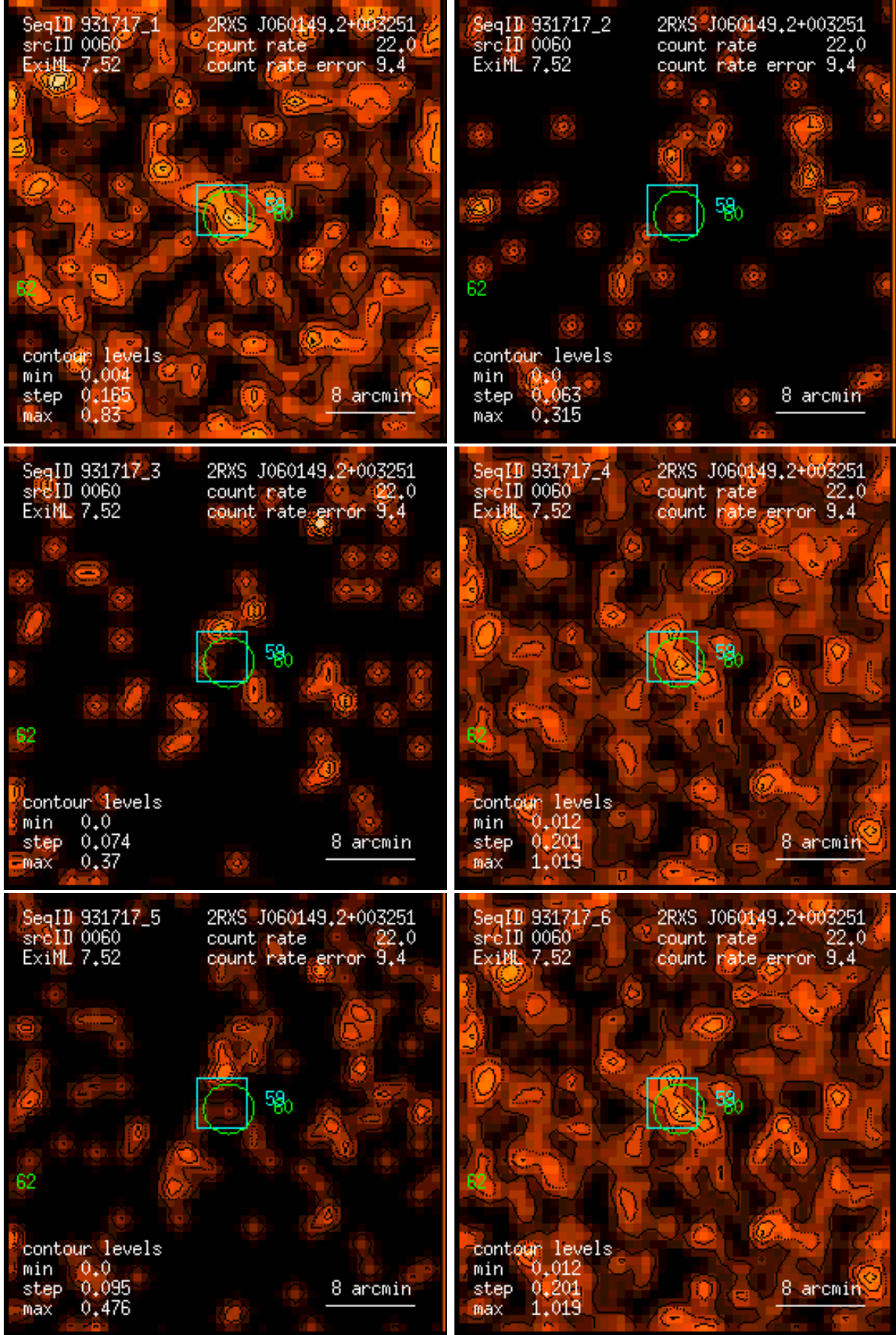
Figure 60: RASS 931717: detection 0060: band rate images, Gaussian filter: (1) PSPC channels 11 – 41, (2) 52 – 90, (3) 91 – 201, (4) 11 – 235, (5) 52 – 201, (6) 11 – 201. Broad band rates in counts/ks. Band rate contour levels in counts/ks/arcmin 2 .
