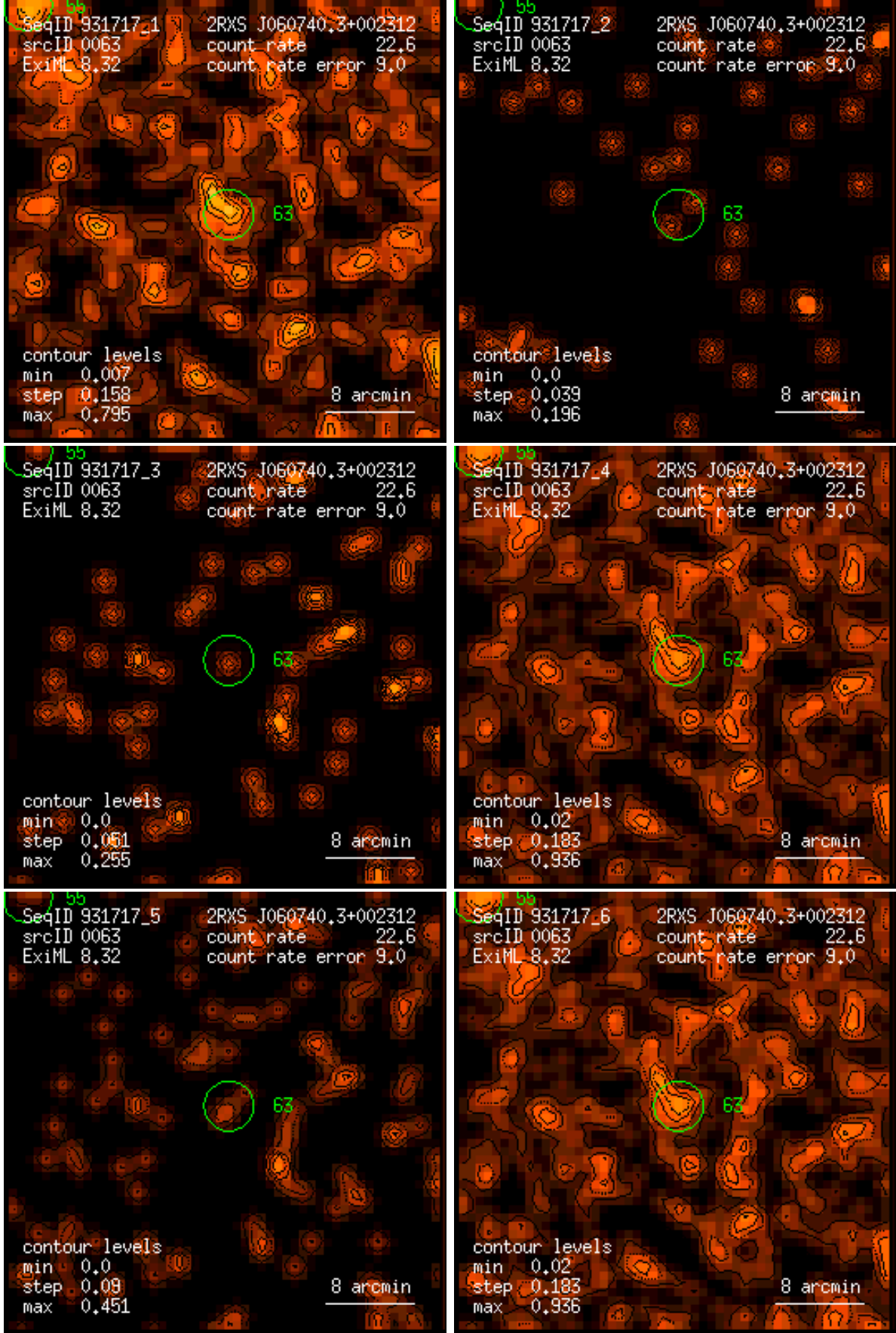
Figure 63: RASS 931717: detection 0063: band rate images, Gaussian filter: (1) PSPC channels 11 – 41, (2) 52 – 90, (3) 91 – 201, (4) 11 – 235, (5) 52 – 201, (6) 11 – 201. Broad band rates in counts/ks. Band rate contour levels in counts/ks/arcmin 2 .
