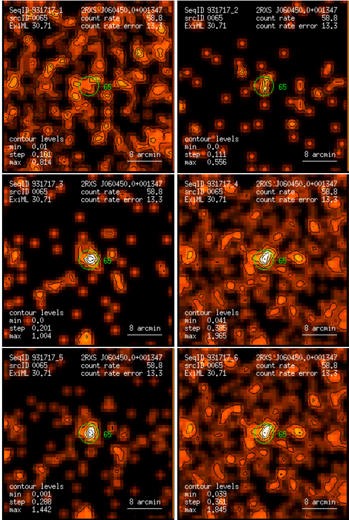
Figure 65: RASS 931717: detection 0065: band rate images, Gaussian filter: (1) PSPC channels 11 – 41, (2) 52 – 90, (3) 91 – 201, (4) 11 – 235, (5) 52 – 201, (6) 11 – 201. Broad band rates in counts/ks. Band rate contour levels in counts/ks/arcmin 2 .
