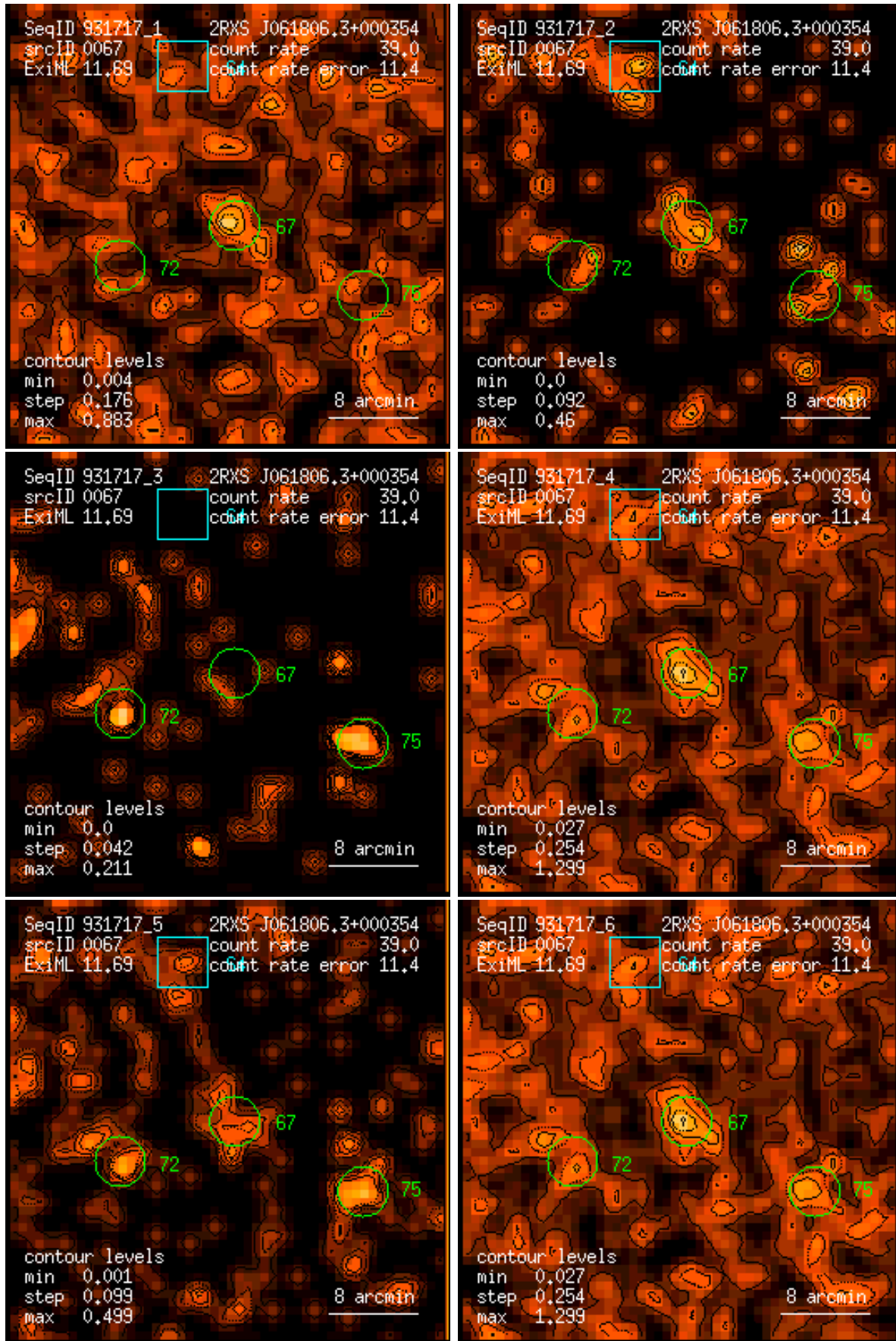
Figure 67: RASS 931717: detection 0067: band rate images, Gaussian filter: (1) PSPC channels 11 – 41, (2) 52 – 90, (3) 91 – 201, (4) 11 – 235, (5) 52 – 201, (6) 11 – 201. Broad band rates in counts/ks. Band rate contour levels in counts/ks/arcmin 2 .
