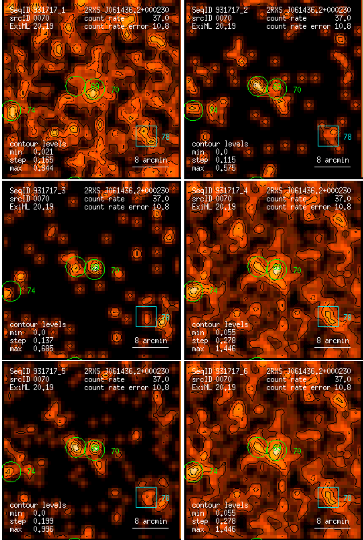
Figure 70: RASS 931717: detection 0070: band rate images, Gaussian filter: (1) PSPC channels 11 – 41, (2) 52 – 90, (3) 91 – 201, (4) 11 – 235, (5) 52 – 201, (6) 11 – 201. Broad band rates in counts/ks. Band rate contour levels in counts/ks/arcmin 2 .
