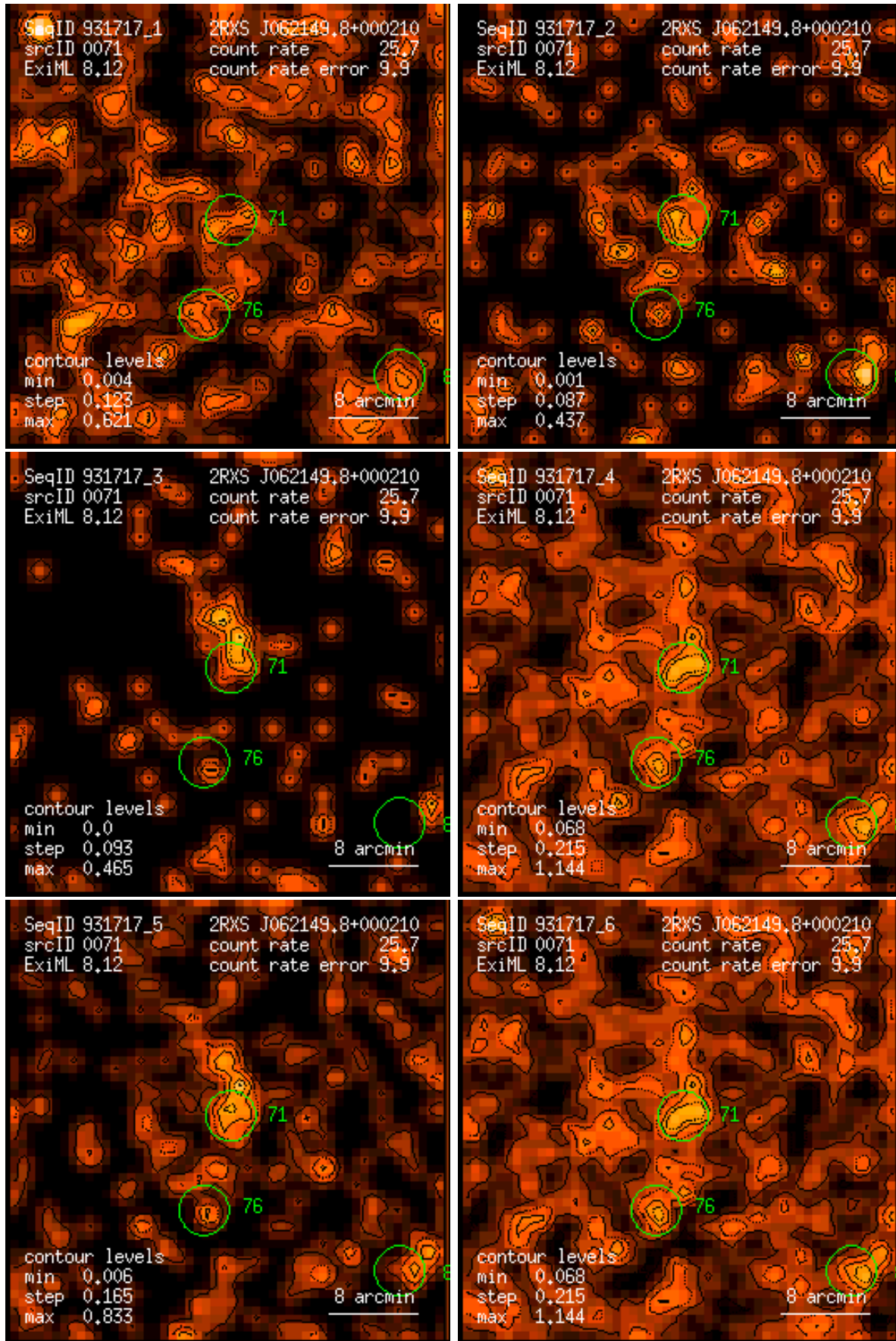
Figure 71: RASS 931717: detection 0071: band rate images, Gaussian filter: (1) PSPC channels 11 – 41, (2) 52 – 90, (3) 91 – 201, (4) 11 – 235, (5) 52 – 201, (6) 11 – 201. Broad band rates in counts/ks. Band rate contour levels in counts/ks/arcmin 2 .
