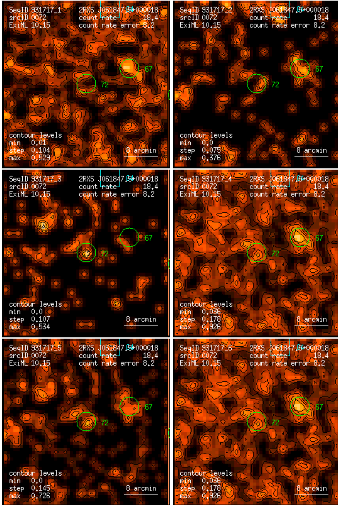
Figure 72: RASS 931717: detection 0072: band rate images, Gaussian filter: (1) PSPC channels 11 – 41, (2) 52 – 90, (3) 91 – 201, (4) 11 – 235, (5) 52 – 201, (6) 11 – 201. Broad band rates in counts/ks. Band rate contour levels in counts/ks/arcmin 2 .
