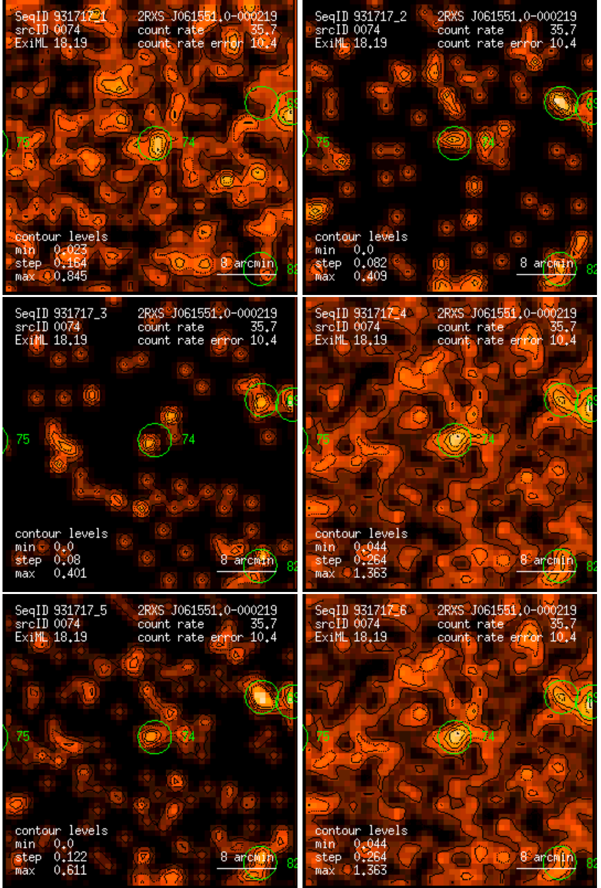
Figure 74: RASS 931717: detection 0074: band rate images, Gaussian filter: (1) PSPC channels 11 – 41, (2) 52 – 90, (3) 91 – 201, (4) 11 – 235, (5) 52 – 201, (6) 11 – 201. Broad band rates in counts/ks. Band rate contour levels in counts/ks/arcmin 2 .
