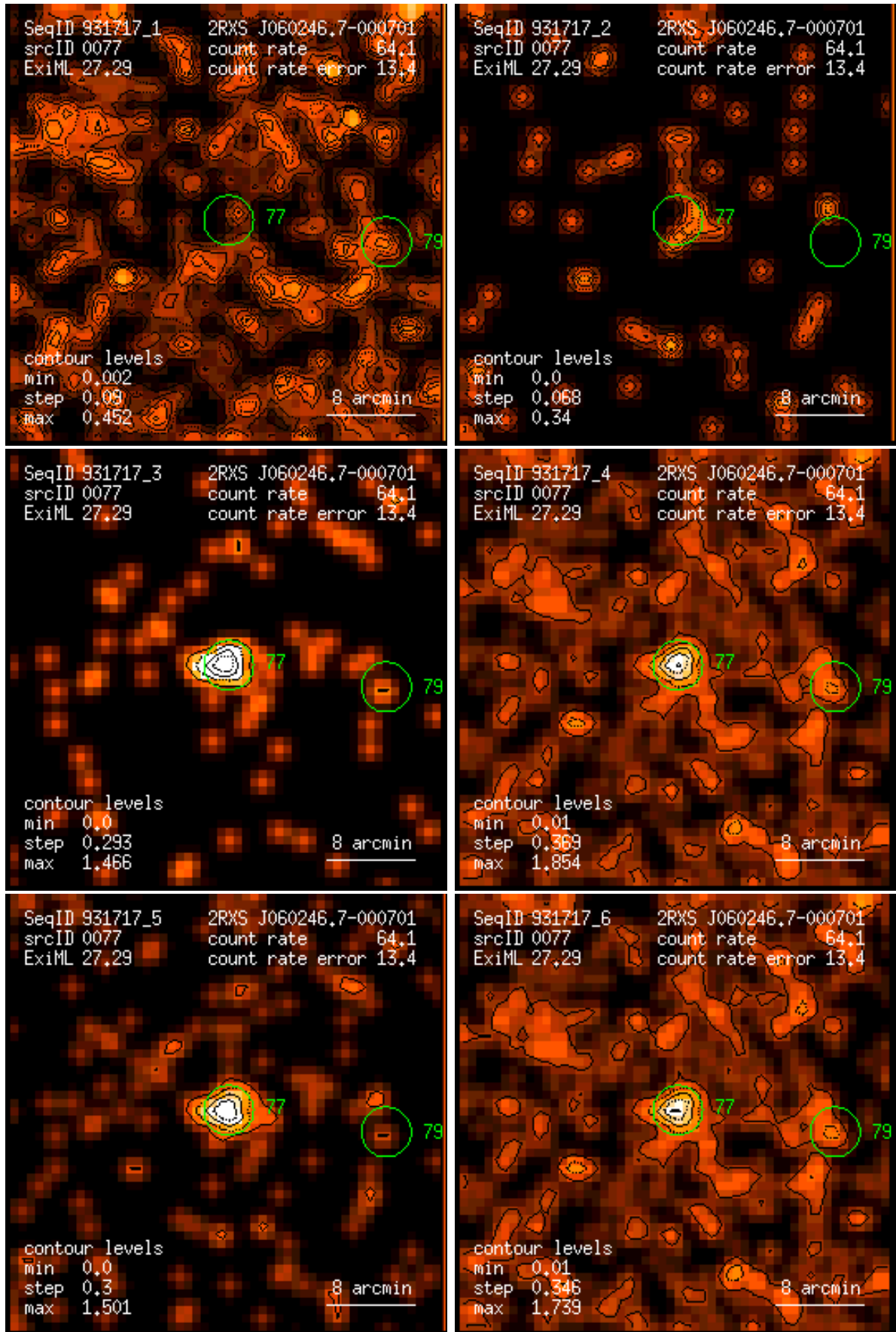
Figure 77: RASS 931717: detection 0077: band rate images, Gaussian filter: (1) PSPC channels 11 – 41, (2) 52 – 90, (3) 91 – 201, (4) 11 – 235, (5) 52 – 201, (6) 11 – 201. Broad band rates in counts/ks. Band rate contour levels in counts/ks/arcmin 2 .
