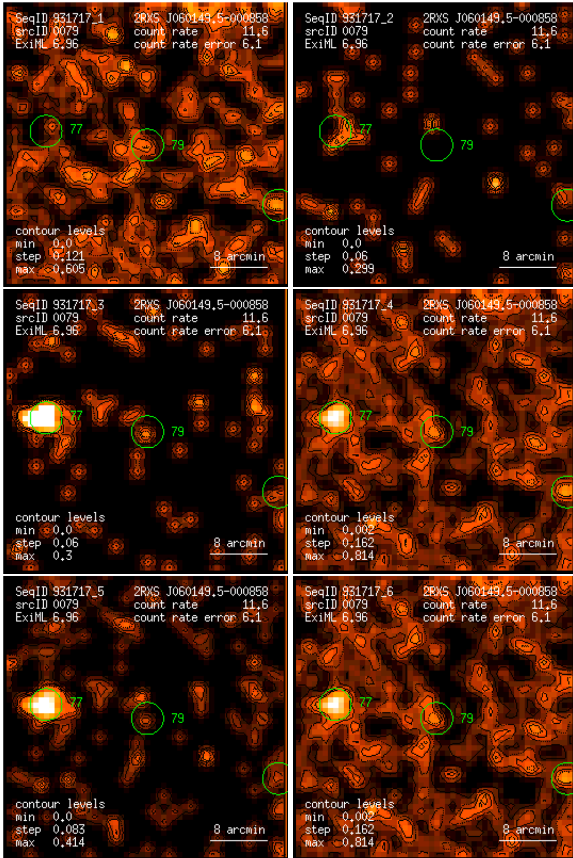
Figure 79: RASS 931717: detection 0079: band rate images, Gaussian filter: (1) PSPC channels 11 – 41, (2) 52 – 90, (3) 91 – 201, (4) 11 – 235, (5) 52 – 201, (6) 11 – 201. Broad band rates in counts/ks. Band rate contour levels in counts/ks/arcmin 2 .
