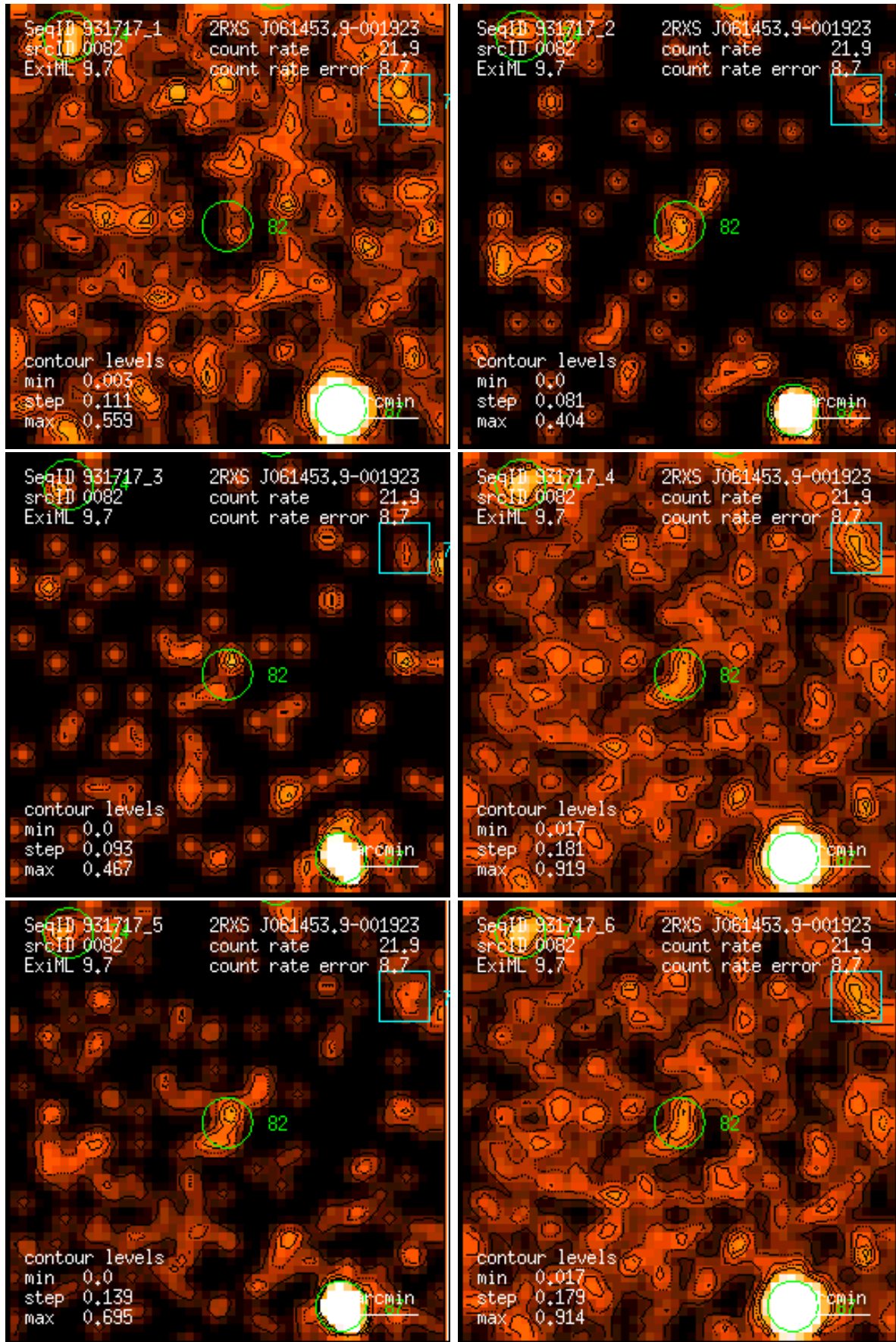
Figure 82: RASS 931717: detection 0082: band rate images, Gaussian filter: (1) PSPC channels 11 – 41, (2) 52 – 90, (3) 91 – 201, (4) 11 – 235, (5) 52 – 201, (6) 11 – 201. Broad band rates in counts/ks. Band rate contour levels in counts/ks/arcmin 2 .
