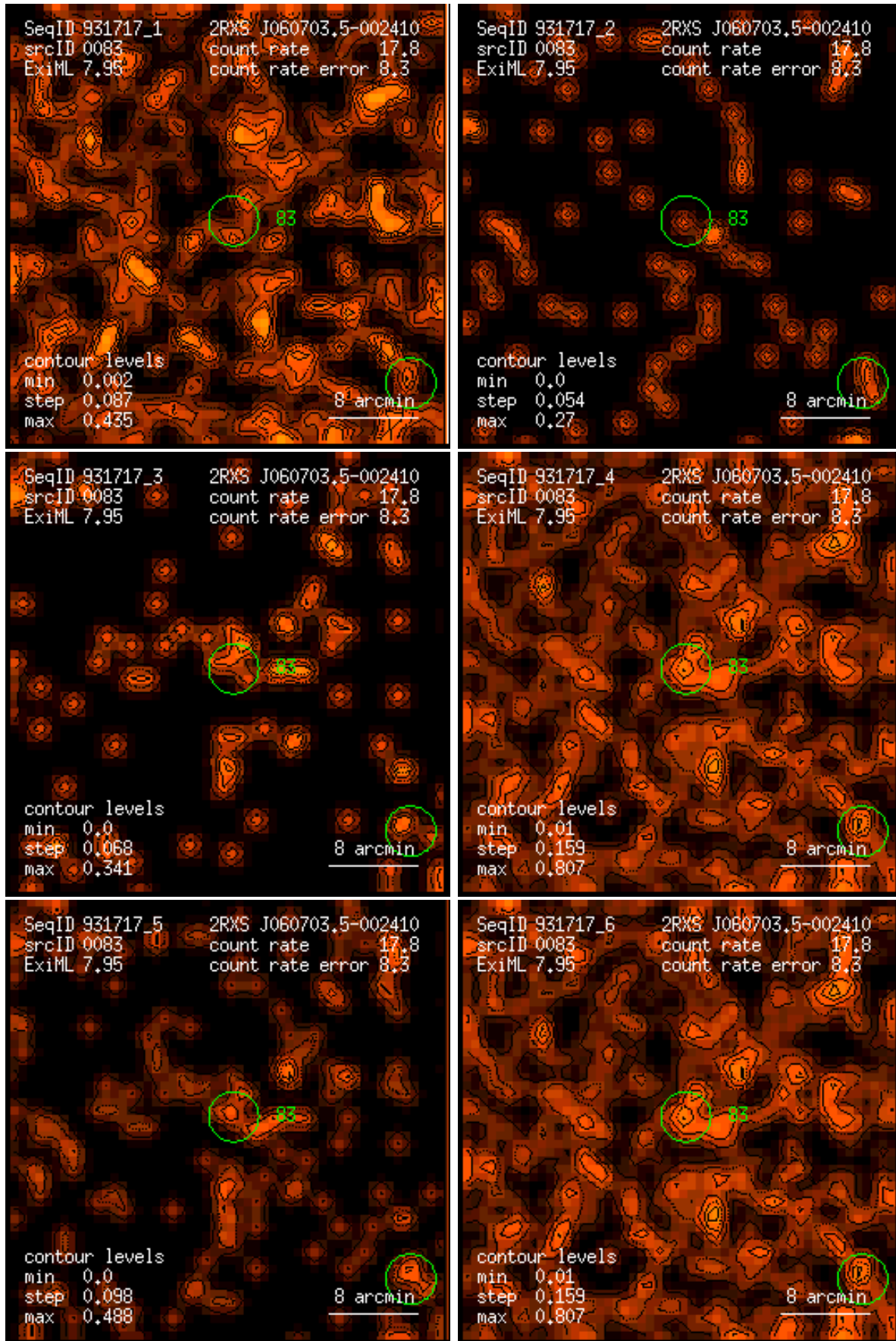
Figure 83: RASS 931717: detection 0083: band rate images, Gaussian filter: (1) PSPC channels 11 – 41, (2) 52 – 90, (3) 91 – 201, (4) 11 – 235, (5) 52 – 201, (6) 11 – 201. Broad band rates in counts/ks. Band rate contour levels in counts/ks/arcmin 2 .
