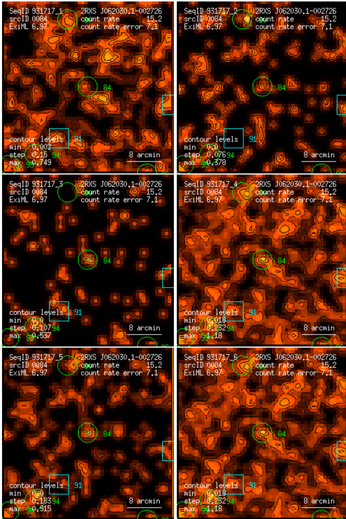
Figure 84: RASS 931717: detection 0084: band rate images, Gaussian filter: (1) PSPC channels 11 – 41, (2) 52 – 90, (3) 91 – 201, (4) 11 – 235, (5) 52 – 201, (6) 11 – 201. Broad band rates in counts/ks. Band rate contour levels in counts/ks/arcmin 2 .
