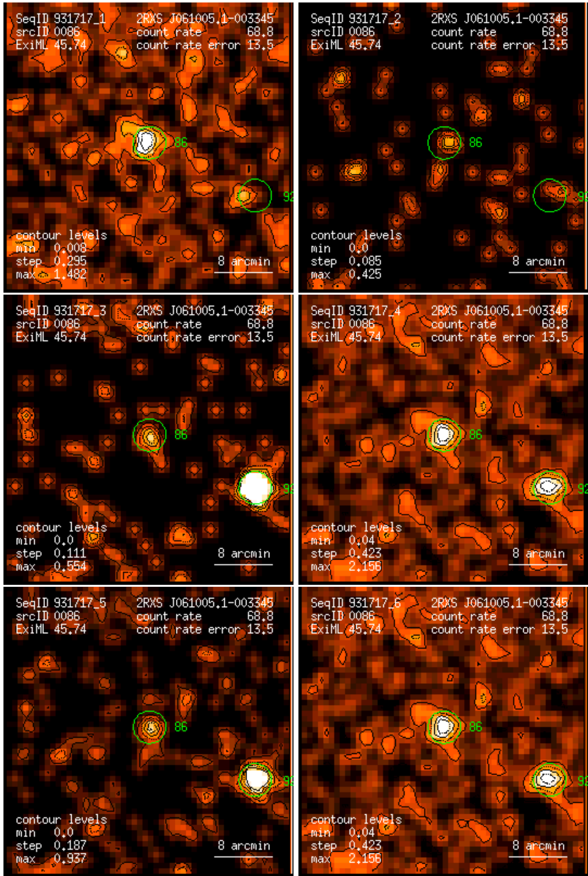
Figure 86: RASS 931717: detection 0086: band rate images, Gaussian filter: (1) PSPC channels 11 – 41, (2) 52 – 90, (3) 91 – 201, (4) 11 – 235, (5) 52 – 201, (6) 11 – 201. Broad band rates in counts/ks. Band rate contour levels in counts/ks/arcmin 2 .
