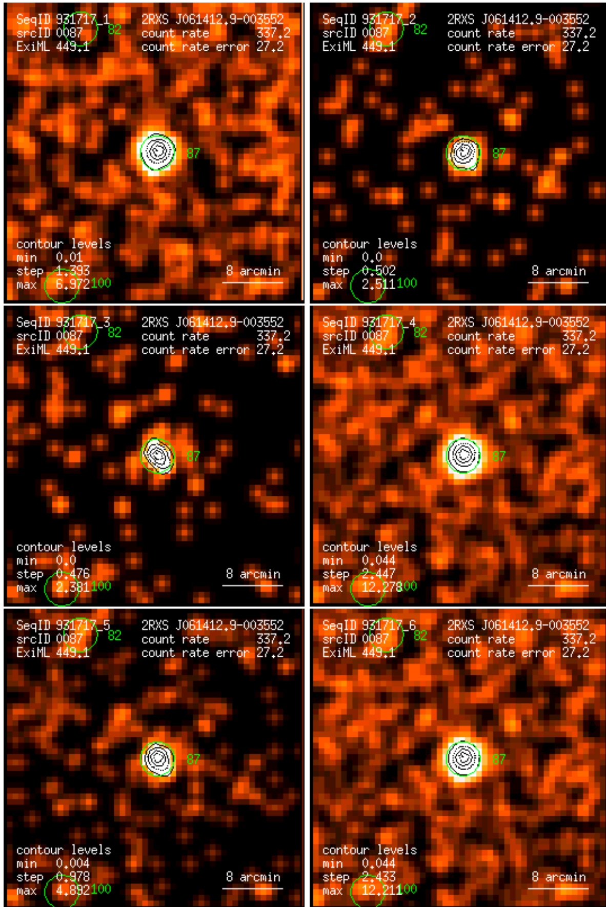
Figure 87: RASS 931717: detection 0087: band rate images, Gaussian filter: (1) PSPC channels 11 – 41, (2) 52 – 90, (3) 91 – 201, (4) 11 – 235, (5) 52 – 201, (6) 11 – 201. Broad band rates in counts/ks. Band rate contour levels in counts/ks/arcmin 2 .
