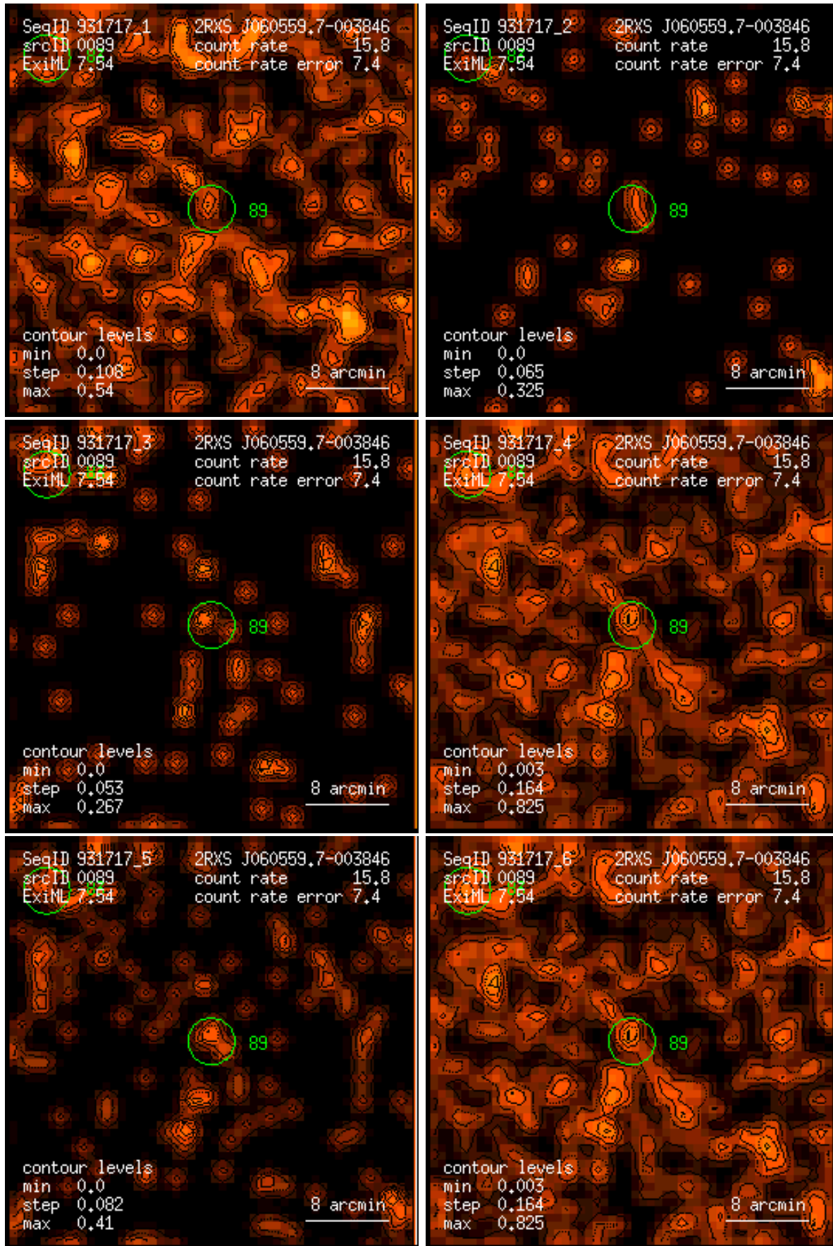
Figure 89: RASS 931717: detection 0089: band rate images, Gaussian filter: (1) PSPC channels 11 – 41, (2) 52 – 90, (3) 91 – 201, (4) 11 – 235, (5) 52 – 201, (6) 11 – 201. Broad band rates in counts/ks. Band rate contour levels in counts/ks/arcmin 2 .
