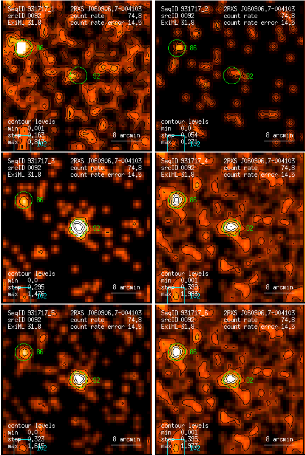
Figure 92: RASS 931717: detection 0092: band rate images, Gaussian filter: (1) PSPC channels 11 – 41, (2) 52 – 90, (3) 91 – 201, (4) 11 – 235, (5) 52 – 201, (6) 11 – 201. Broad band rates in counts/ks. Band rate contour levels in counts/ks/arcmin 2 .
