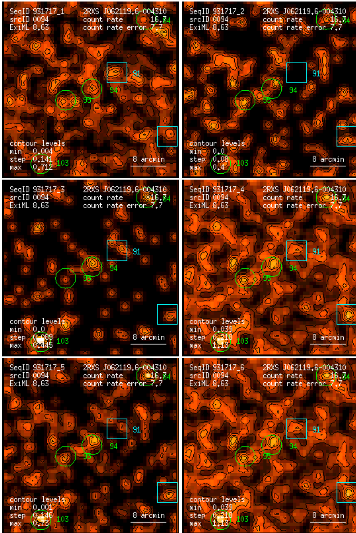
Figure 94: RASS 931717: detection 0094: band rate images, Gaussian filter: (1) PSPC channels 11 – 41, (2) 52 – 90, (3) 91 – 201, (4) 11 – 235, (5) 52 – 201, (6) 11 – 201. Broad band rates in counts/ks. Band rate contour levels in counts/ks/arcmin 2 .
