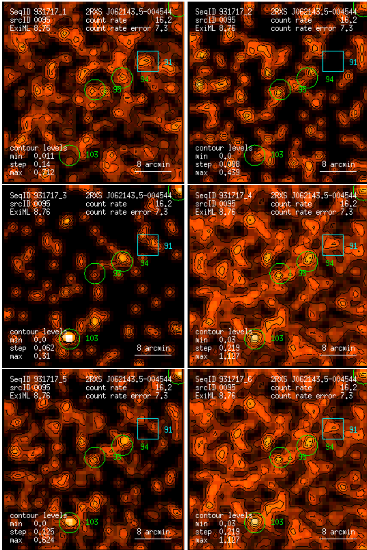
Figure 95: RASS 931717: detection 0095: band rate images, Gaussian filter: (1) PSPC channels 11 – 41, (2) 52 – 90, (3) 91 – 201, (4) 11 – 235, (5) 52 – 201, (6) 11 – 201. Broad band rates in counts/ks. Band rate contour levels in counts/ks/arcmin 2 .
