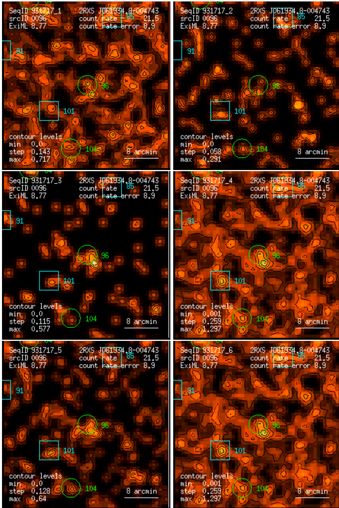
Figure 96: RASS 931717: detection 0096: band rate images, Gaussian filter: (1) PSPC channels 11 – 41, (2) 52 – 90, (3) 91 – 201, (4) 11 – 235, (5) 52 – 201, (6) 11 – 201. Broad band rates in counts/ks. Band rate contour levels in counts/ks/arcmin 2 .
