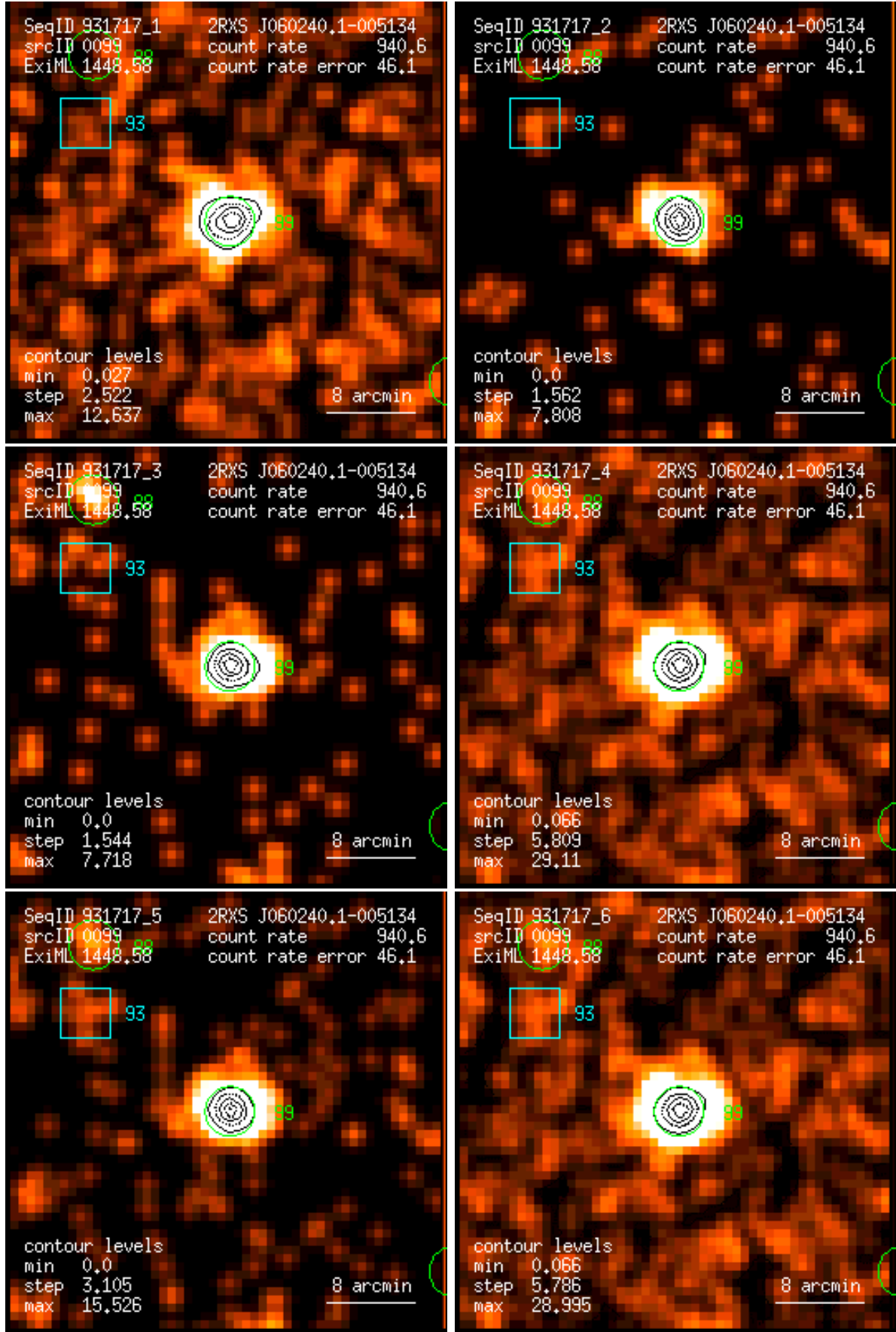
Figure 99: RASS 931717: detection 0099: band rate images, Gaussian filter: (1) PSPC channels 11 – 41, (2) 52 – 90, (3) 91 – 201, (4) 11 – 235, (5) 52 – 201, (6) 11 – 201. Broad band rates in counts/ks. Band rate contour levels in counts/ks/arcmin 2 .
