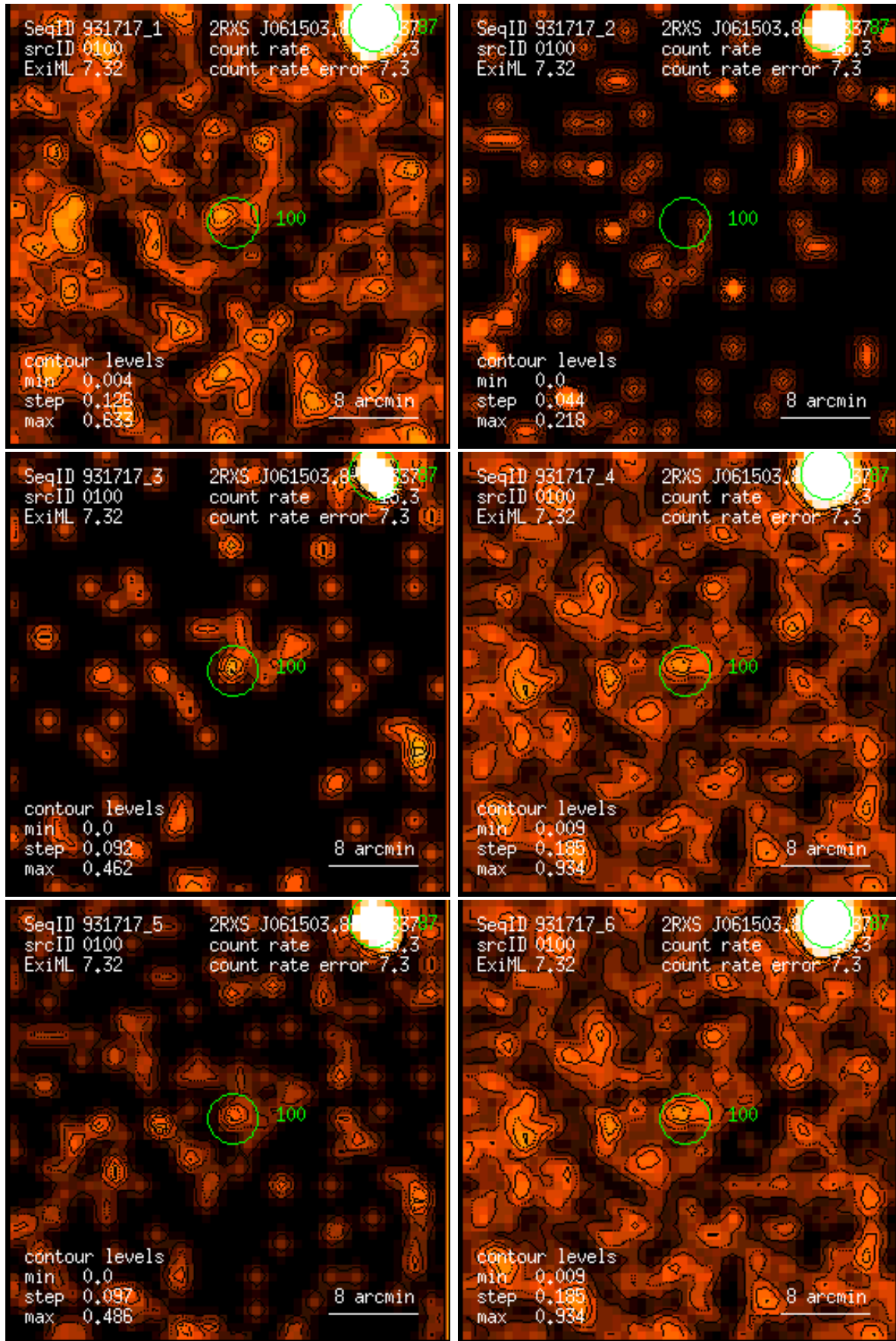
Figure 100: RASS 931717: detection 0100: band rate images, Gaussian filter: (1) PSPC channels 11 – 41, (2) 52 – 90, (3) 91 – 201, (4) 11 – 235, (5) 52 – 201, (6) 11 – 201. Broad band rates in counts/ks. Band rate contour levels in counts/ks/arcmin 2 .
