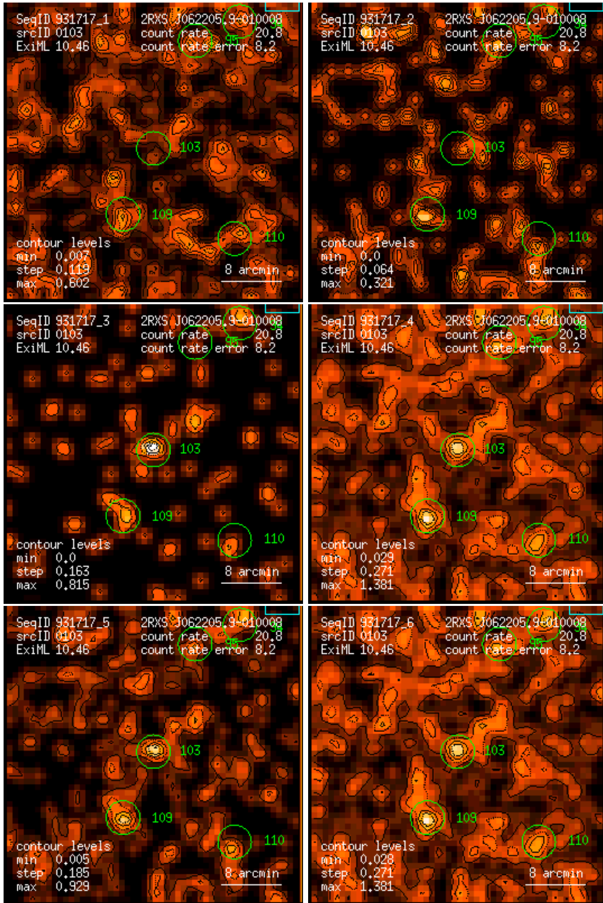
Figure 103: RASS 931717: detection 0103: band rate images, Gaussian filter: (1) PSPC channels 11 – 41, (2) 52 – 90, (3) 91 – 201, (4) 11 – 235, (5) 52 – 201, (6) 11 – 201. Broad band rates in counts/ks. Band rate contour levels in counts/ks/arcmin 2 .
