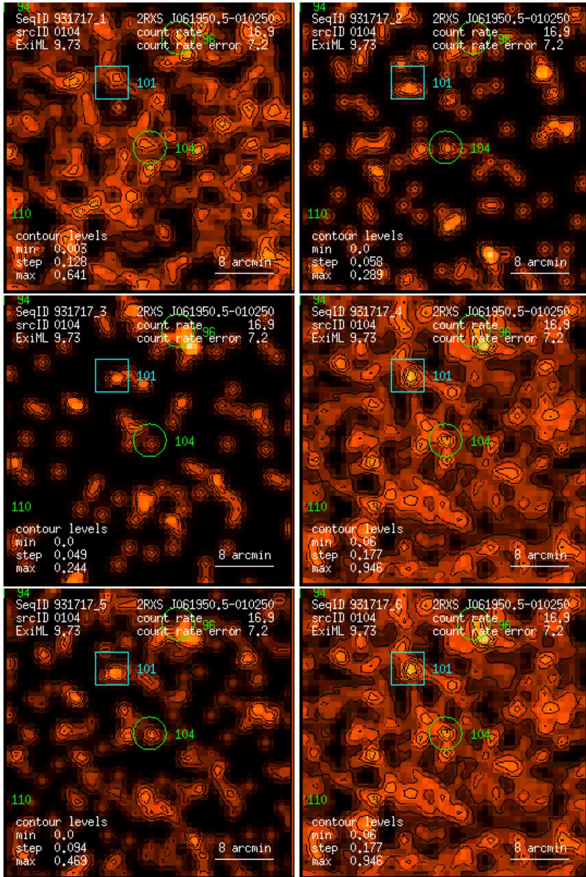
Figure 104: RASS 931717: detection 0104: band rate images, Gaussian filter: (1) PSPC channels 11 – 41, (2) 52 – 90, (3) 91 – 201, (4) 11 – 235, (5) 52 – 201, (6) 11 – 201. Broad band rates in counts/ks. Band rate contour levels in counts/ks/arcmin 2 .
