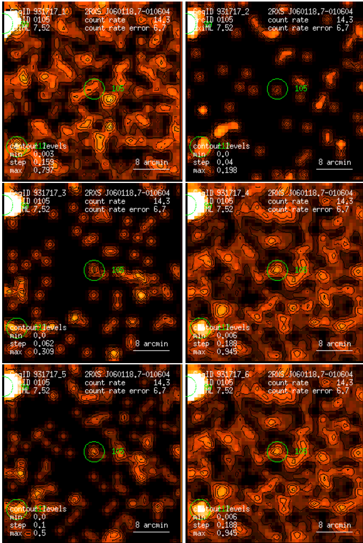
Figure 105: RASS 931717: detection 0105: band rate images, Gaussian filter: (1) PSPC channels 11 – 41, (2) 52 – 90, (3) 91 – 201, (4) 11 – 235, (5) 52 – 201, (6) 11 – 201. Broad band rates in counts/ks. Band rate contour levels in counts/ks/arcmin 2 .
