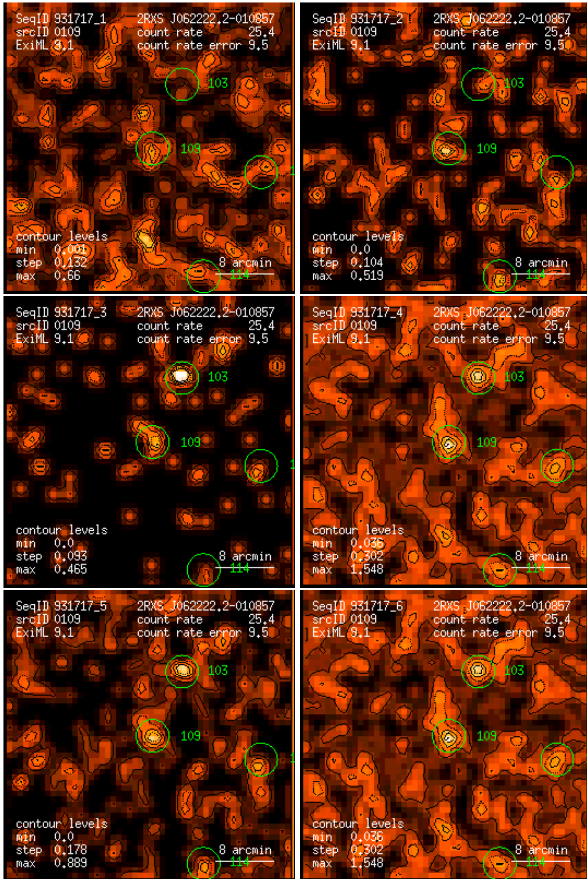
Figure 109: RASS 931717: detection 0109: band rate images, Gaussian filter: (1) PSPC channels 11 – 41, (2) 52 – 90, (3) 91 – 201, (4) 11 – 235, (5) 52 – 201, (6) 11 – 201. Broad band rates in counts/ks. Band rate contour levels in counts/ks/arcmin 2 .
