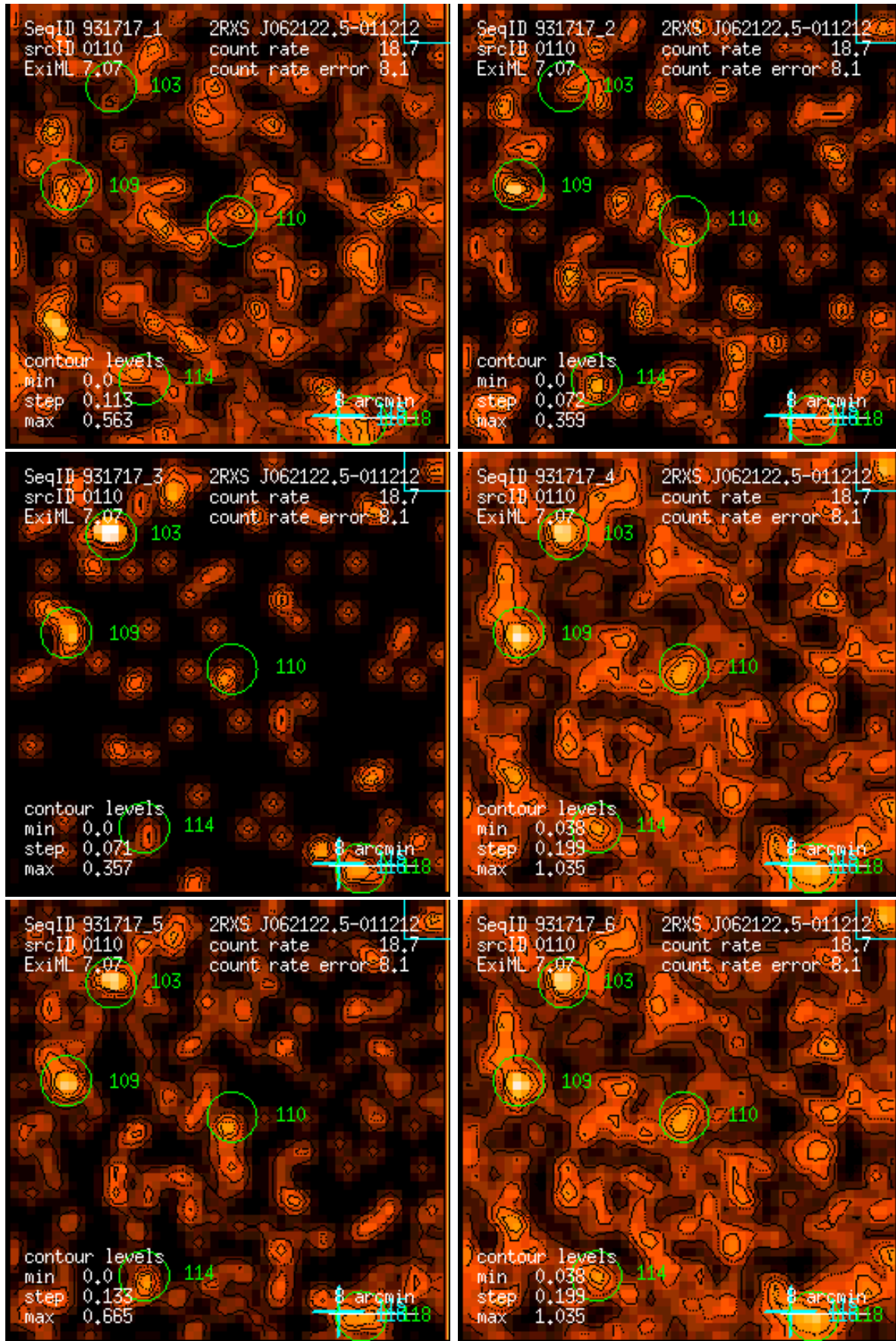
Figure 110: RASS 931717: detection 0110: band rate images, Gaussian filter: (1) PSPC channels 11 – 41, (2) 52 – 90, (3) 91 – 201, (4) 11 – 235, (5) 52 – 201, (6) 11 – 201. Broad band rates in counts/ks. Band rate contour levels in counts/ks/arcmin 2 .
