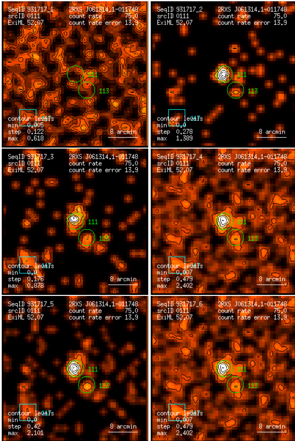
Figure 111: RASS 931717: detection 0111: band rate images, Gaussian filter: (1) PSPC channels 11 – 41, (2) 52 – 90, (3) 91 – 201, (4) 11 – 235, (5) 52 – 201, (6) 11 – 201. Broad band rates in counts/ks. Band rate contour levels in counts/ks/arcmin 2 .
