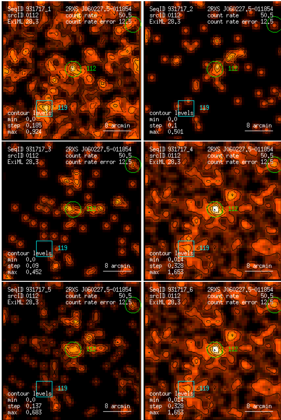
Figure 112: RASS 931717: detection 0112: band rate images, Gaussian filter: (1) PSPC channels 11 – 41, (2) 52 – 90, (3) 91 – 201, (4) 11 – 235, (5) 52 – 201, (6) 11 – 201. Broad band rates in counts/ks. Band rate contour levels in counts/ks/arcmin 2 .
