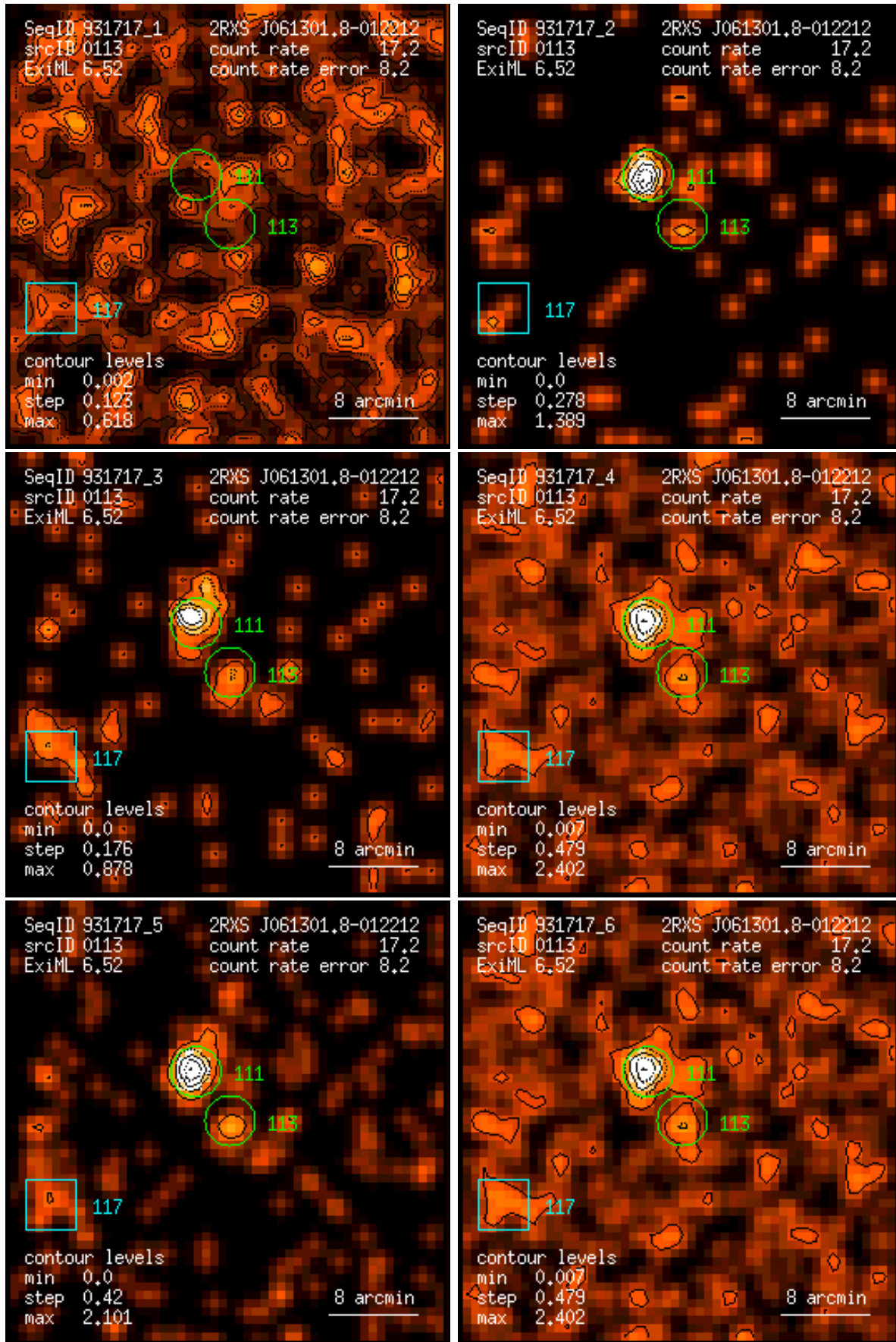
Figure 113: RASS 931717: detection 0113: band rate images, Gaussian filter: (1) PSPC channels 11 – 41, (2) 52 – 90, (3) 91 – 201, (4) 11 – 235, (5) 52 – 201, (6) 11 – 201. Broad band rates in counts/ks. Band rate contour levels in counts/ks/arcmin 2 .
