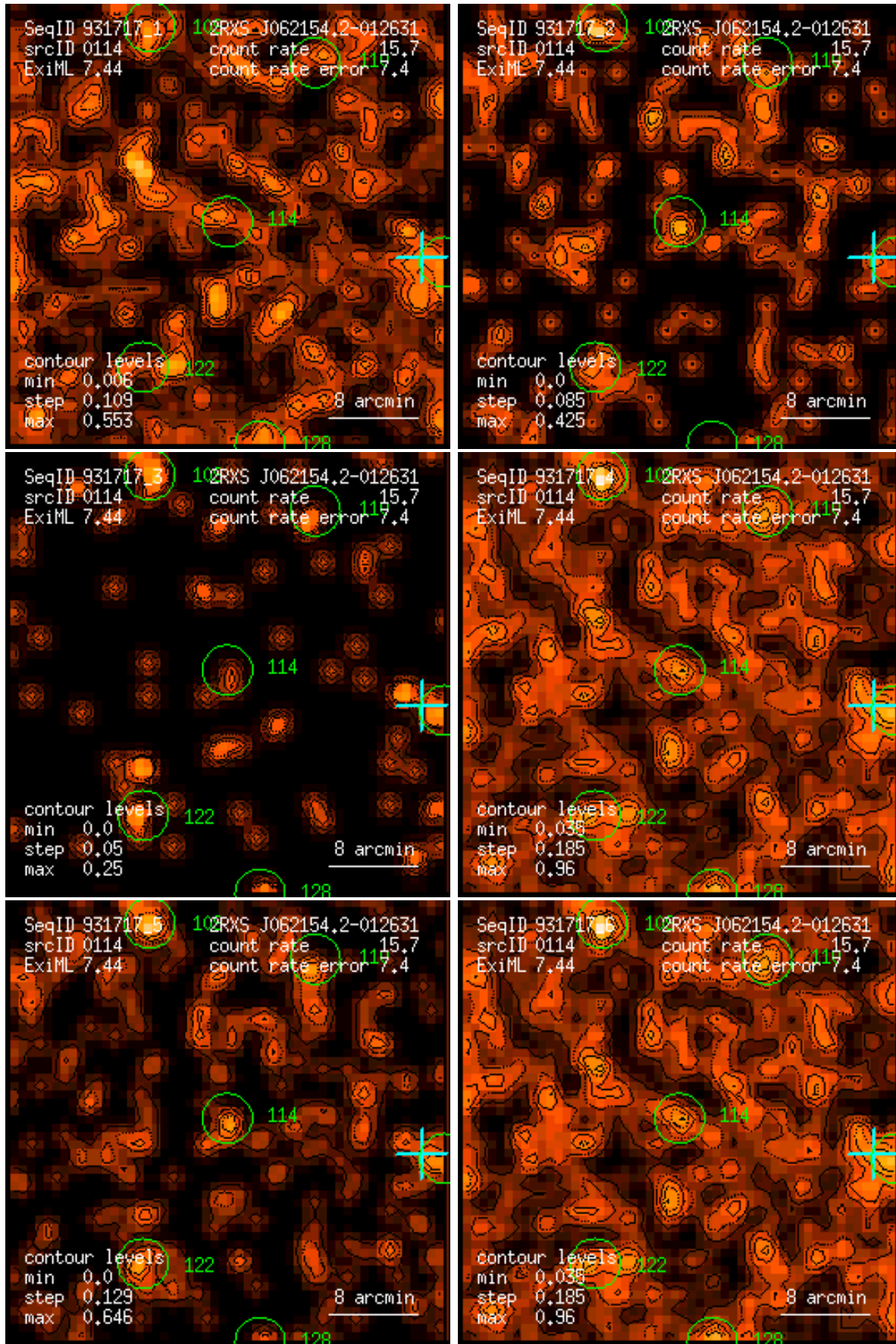
Figure 114: RASS 931717: detection 0114: band rate images, Gaussian filter: (1) PSPC channels 11 – 41, (2) 52 – 90, (3) 91 – 201, (4) 11 – 235, (5) 52 – 201, (6) 11 – 201. Broad band rates in counts/ks. Band rate contour levels in counts/ks/arcmin 2 .
