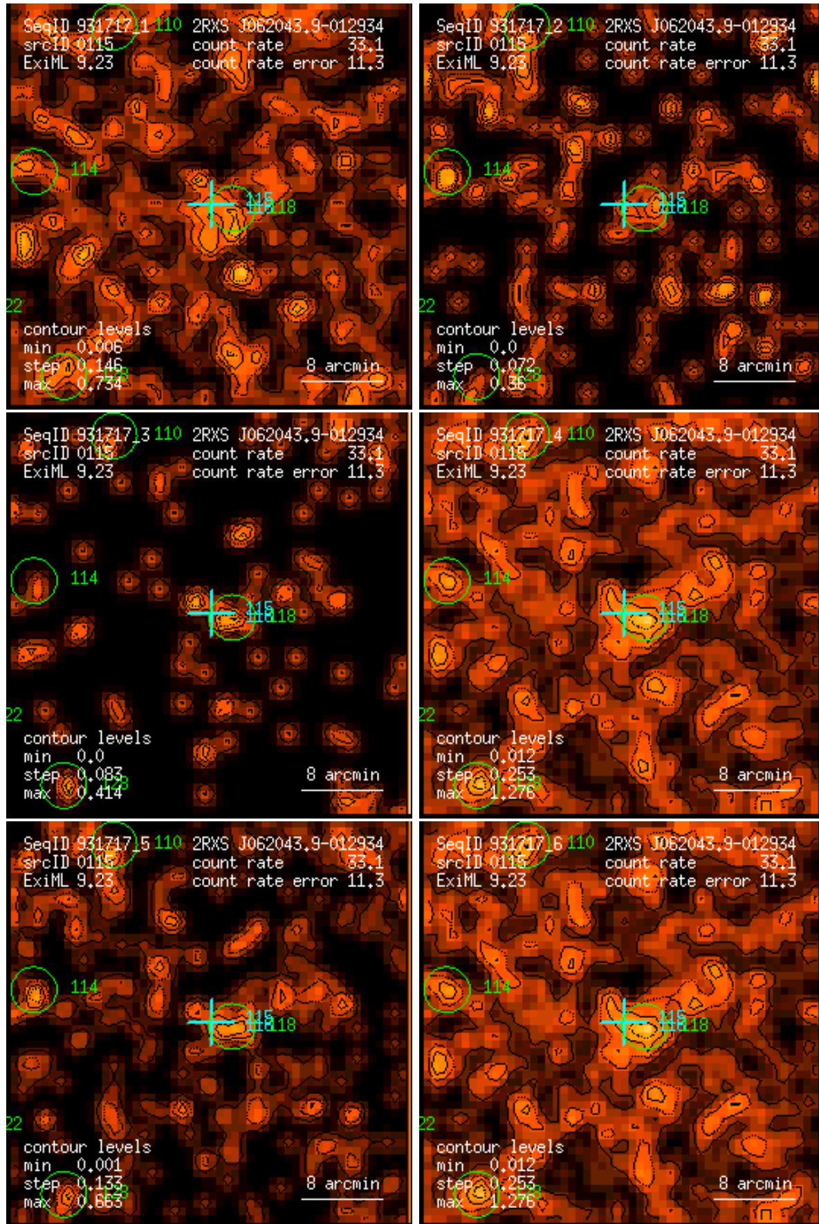
Figure 115: RASS 931717: detection 0115: band rate images, Gaussian filter: (1) PSPPC channels 11 – 41, (2) 52 – 90, (3) 91 – 201, (4) 11 – 235, (5) 52 – 201, (6) 11 – 201. Broad band rates in counts/ks. Band rate contour levels in counts/ks/arcmin 2 .
