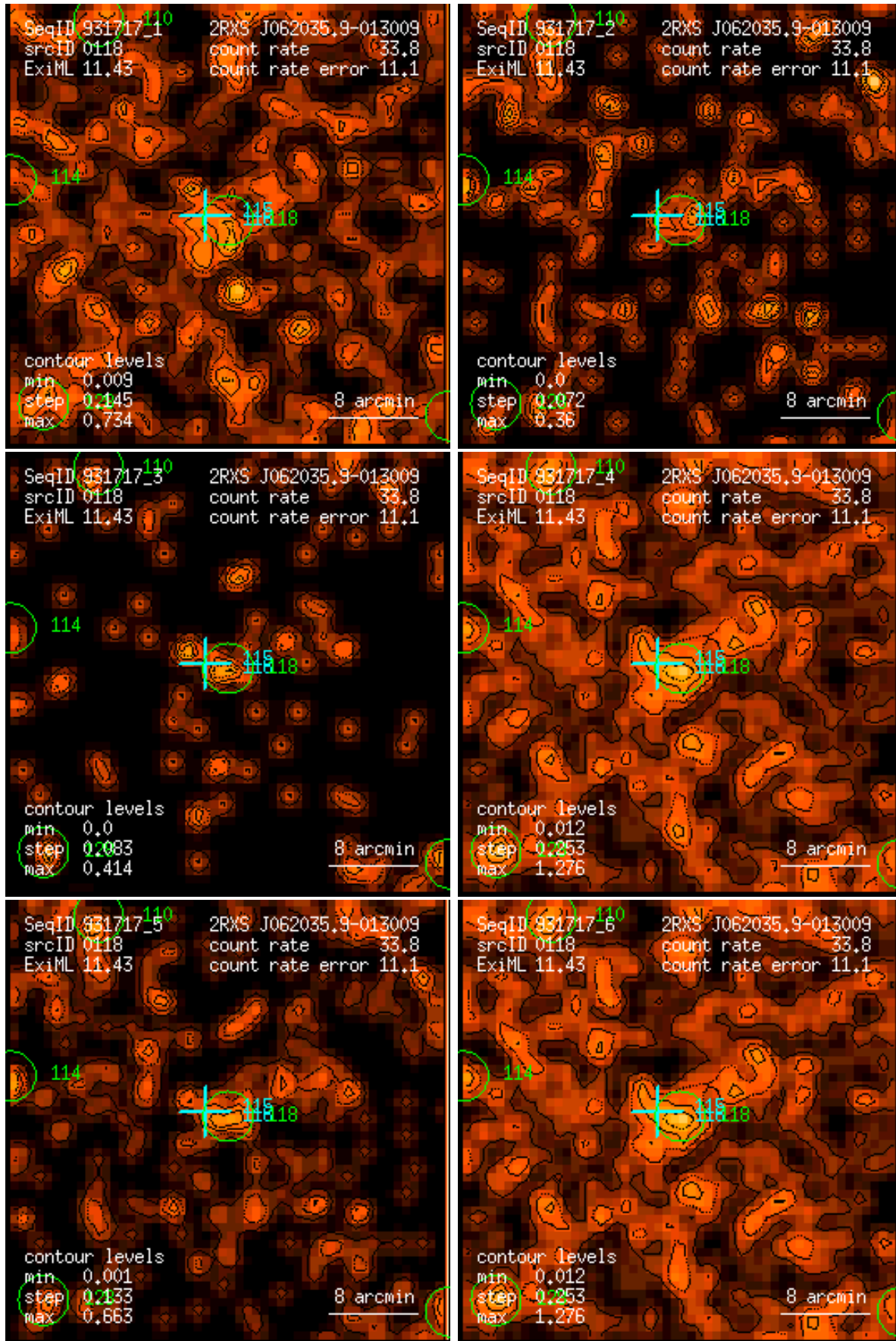
Figure 118: RASS 931717: detection 0118: band rate images, Gaussian filter: (1) PSPC channels 11 – 41, (2) 52 – 90, (3) 91 – 201, (4) 11 – 235, (5) 52 – 201, (6) 11 – 201. Broad band rates in counts/ks. Band rate contour levels in counts/ks/arcmin 2 .
