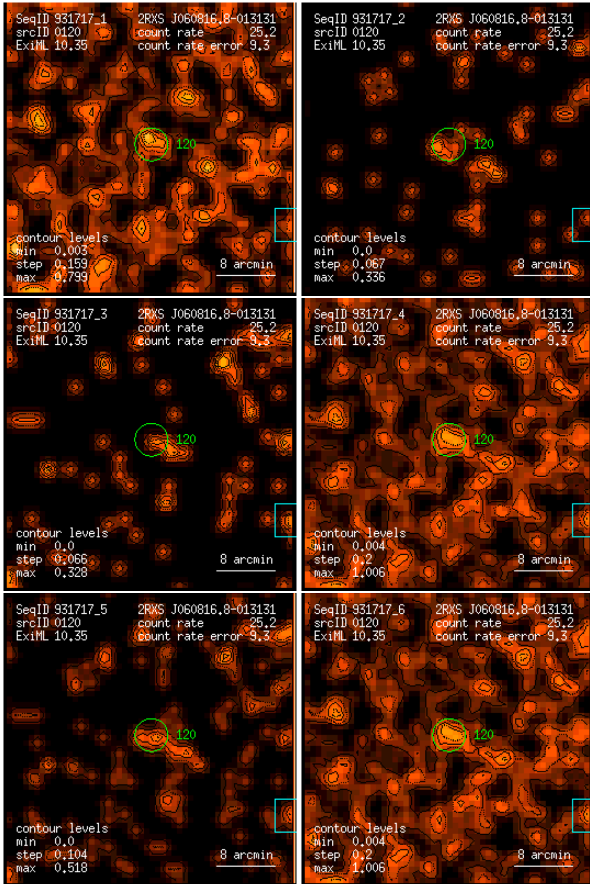
Figure 120: RASS 931717: detection 0120: band rate images, Gaussian filter: (1) PSPC channels 11 – 41, (2) 52 – 90, (3) 91 – 201, (4) 11 – 235, (5) 52 – 201, (6) 11 – 201. Broad band rates in counts/ks. Band rate contour levels in counts/ks/arcmin 2 .
