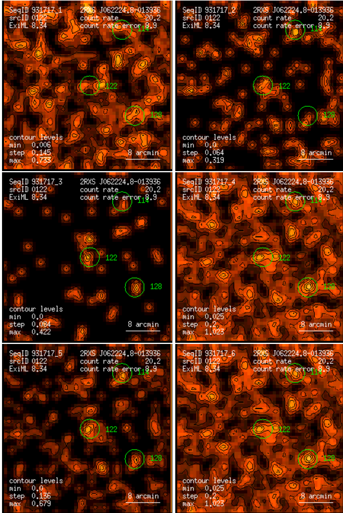
Figure 122: RASS 931717: detection 0122: band rate images, Gaussian filter: (1) PSPC channels 11 – 41, (2) 52 – 90, (3) 91 – 201, (4) 11 – 235, (5) 52 – 201, (6) 11 – 201. Broad band rates in counts/ks. Band rate contour levels in counts/ks/arcmin 2 .
