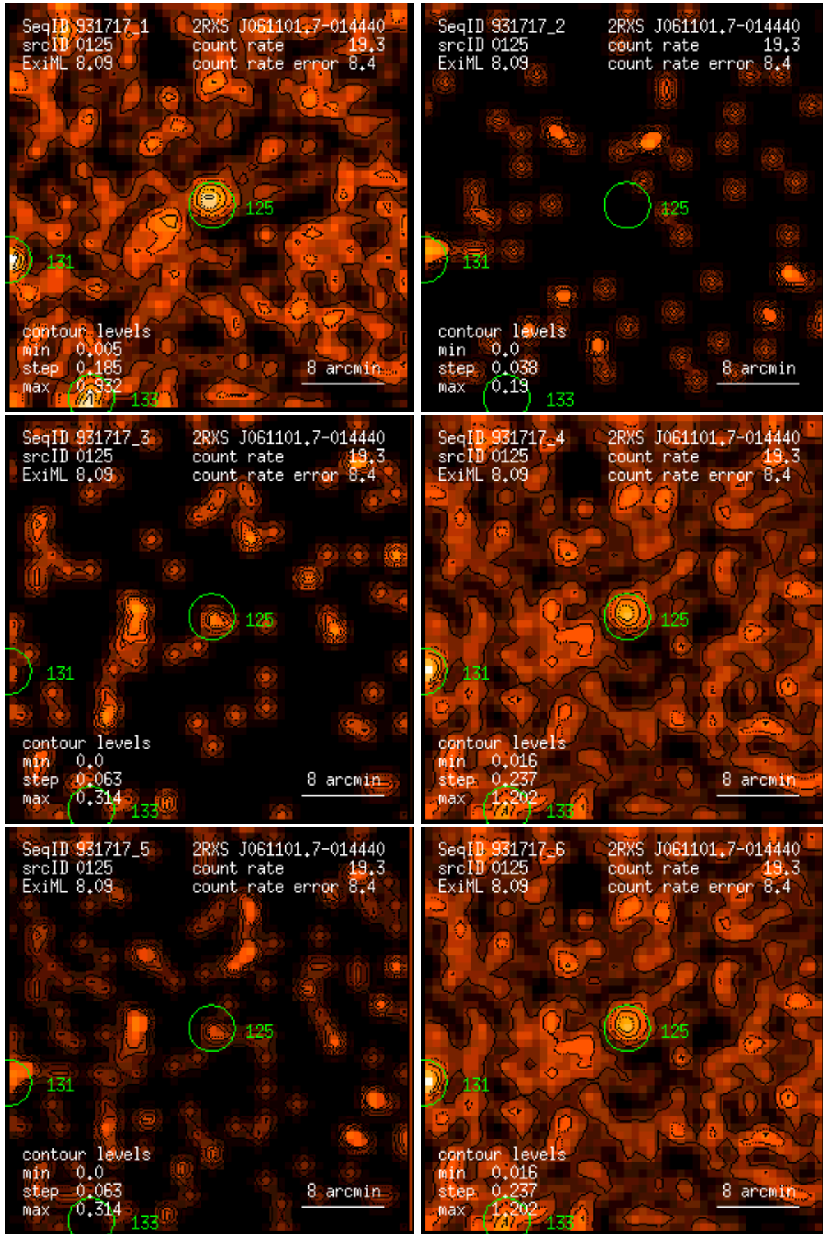
Figure 125: RASS 931717: detection 0125: band rate images, Gaussian filter: (1) PSPC channels 11 – 41, (2) 52 – 90, (3) 91 – 201, (4) 11 – 235, (5) 52 – 201, (6) 11 – 201. Broad band rates in counts/ks. Band rate contour levels in counts/ks/arcmin 2 .
