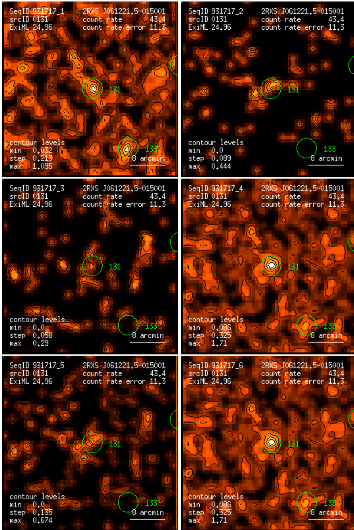
Figure 131: RASS 931717: detection 0131: band rate images, Gaussian filter: (1) PSPC channels 11 – 41, (2) 52 – 90, (3) 91 – 201, (4) 11 – 235, (5) 52 – 201, (6) 11 – 201. Broad band rates in counts/ks. Band rate contour levels in counts/ks/arcmin 2 .
