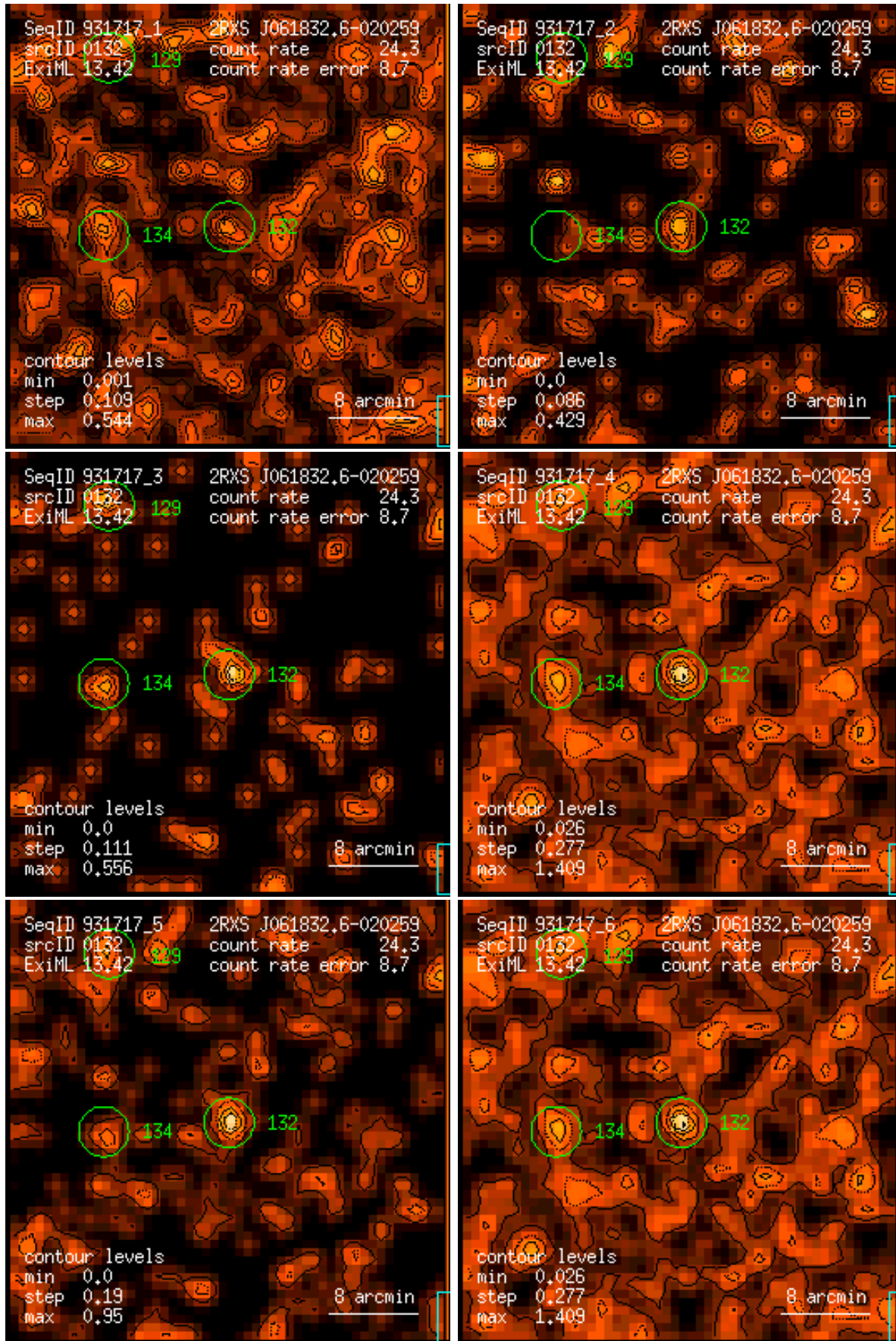
Figure 132: RASS 931717: detection 0132: band rate images, Gaussian filter: (1) PSPC channels 11 – 41, (2) 52 – 90, (3) 91 – 201, (4) 11 – 235, (5) 52 – 201, (6) 11 – 201. Broad band rates in counts/ks. Band rate contour levels in counts/ks/arcmin 2 .
