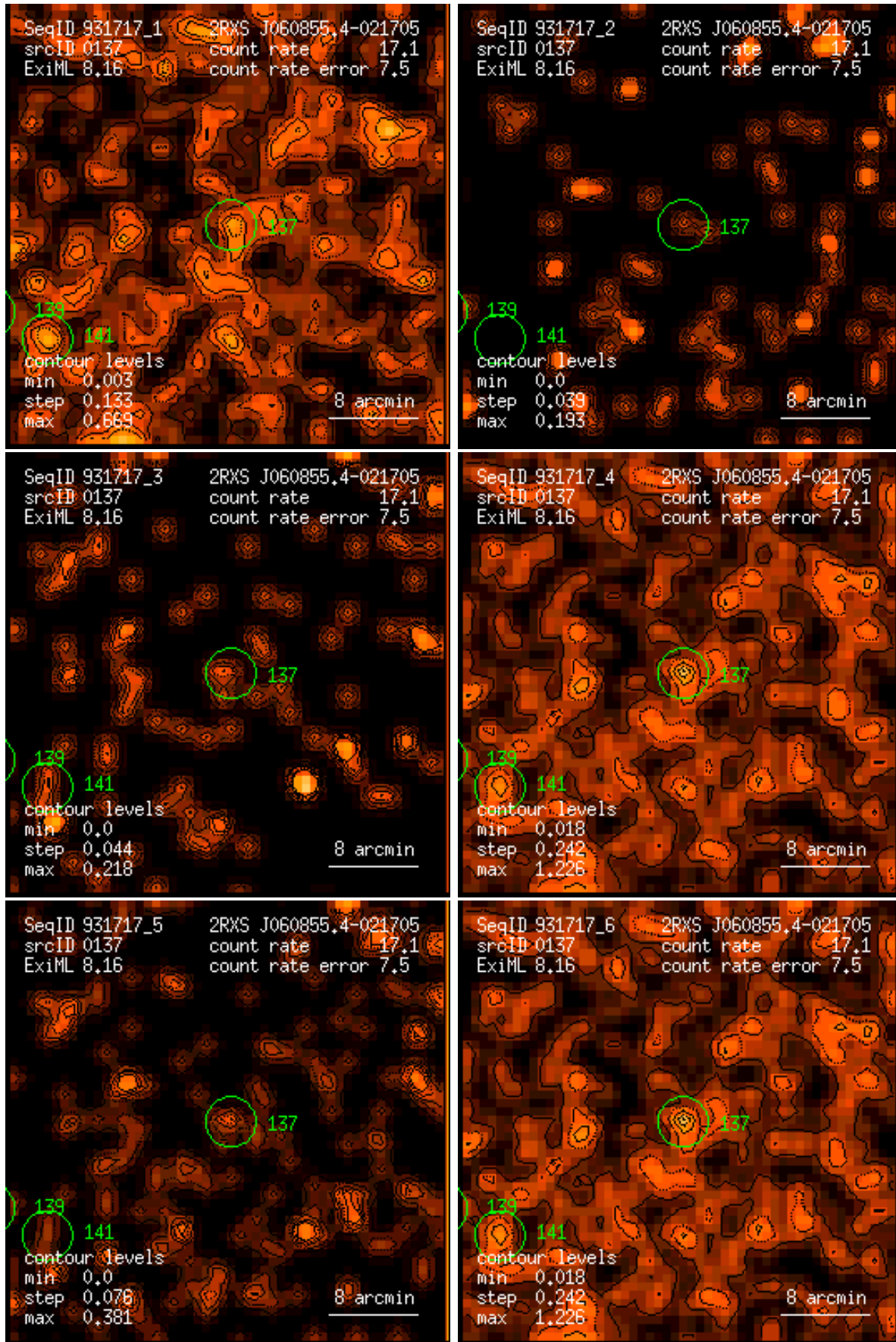
Figure 137: RASS 931717: detection 0137: band rate images, Gaussian filter: (1) PSPC channels 11 – 41, (2) 52 – 90, (3) 91 – 201, (4) 11 – 235, (5) 52 – 201, (6) 11 – 201. Broad band rates in counts/ks. Band rate contour levels in counts/ks/arcmin 2 .
