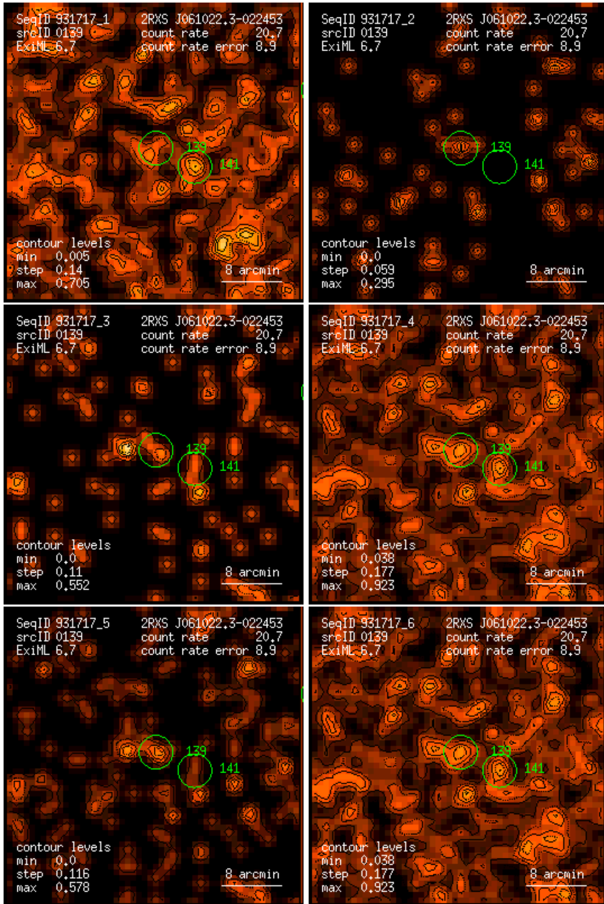
Figure 139: RASS 931717: detection 0139: band rate images, Gaussian filter: (1) PSPC channels 11 – 41, (2) 52 – 90, (3) 91 – 201, (4) 11 – 235, (5) 52 – 201, (6) 11 – 201. Broad band rates in counts/ks. Band rate contour levels in counts/ks/arcmin 2 .
