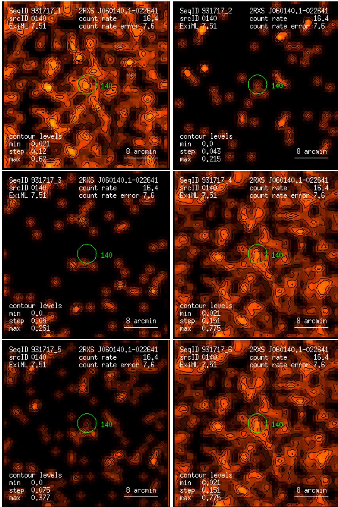
Figure 140: RASS 931717: detection 0140: band rate images, Gaussian filter: (1) PSPC channels 11 – 41, (2) 52 – 90, (3) 91 – 201, (4) 11 – 235, (5) 52 – 201, (6) 11 – 201. Broad band rates in counts/ks. Band rate contour levels in counts/ks/arcmin 2 .
