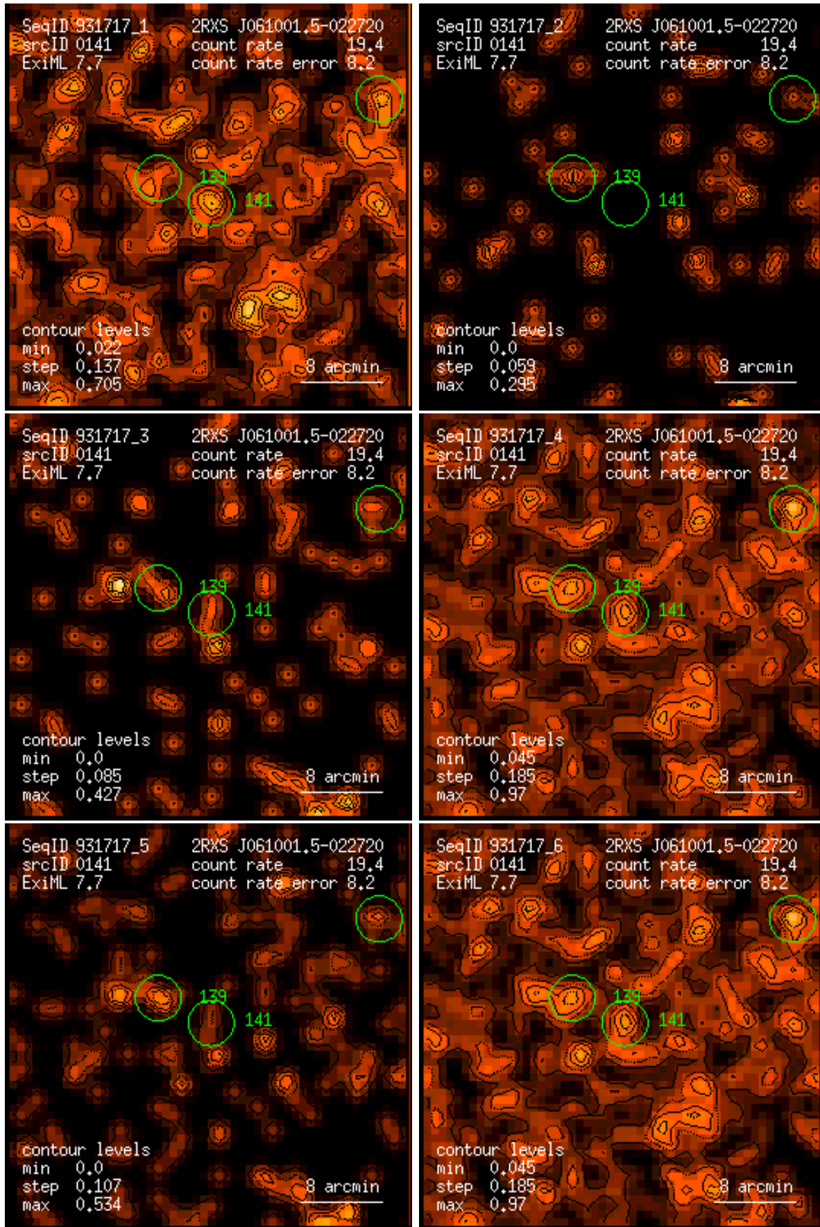
Figure 141: RASS 931717: detection 0141: band rate images, Gaussian filter: (1) PSPC channels 11 – 41, (2) 52 – 90, (3) 91 – 201, (4) 11 – 235, (5) 52 – 201, (6) 11 – 201. Broad band rates in counts/ks. Band rate contour levels in counts/ks/arcmin 2 .
