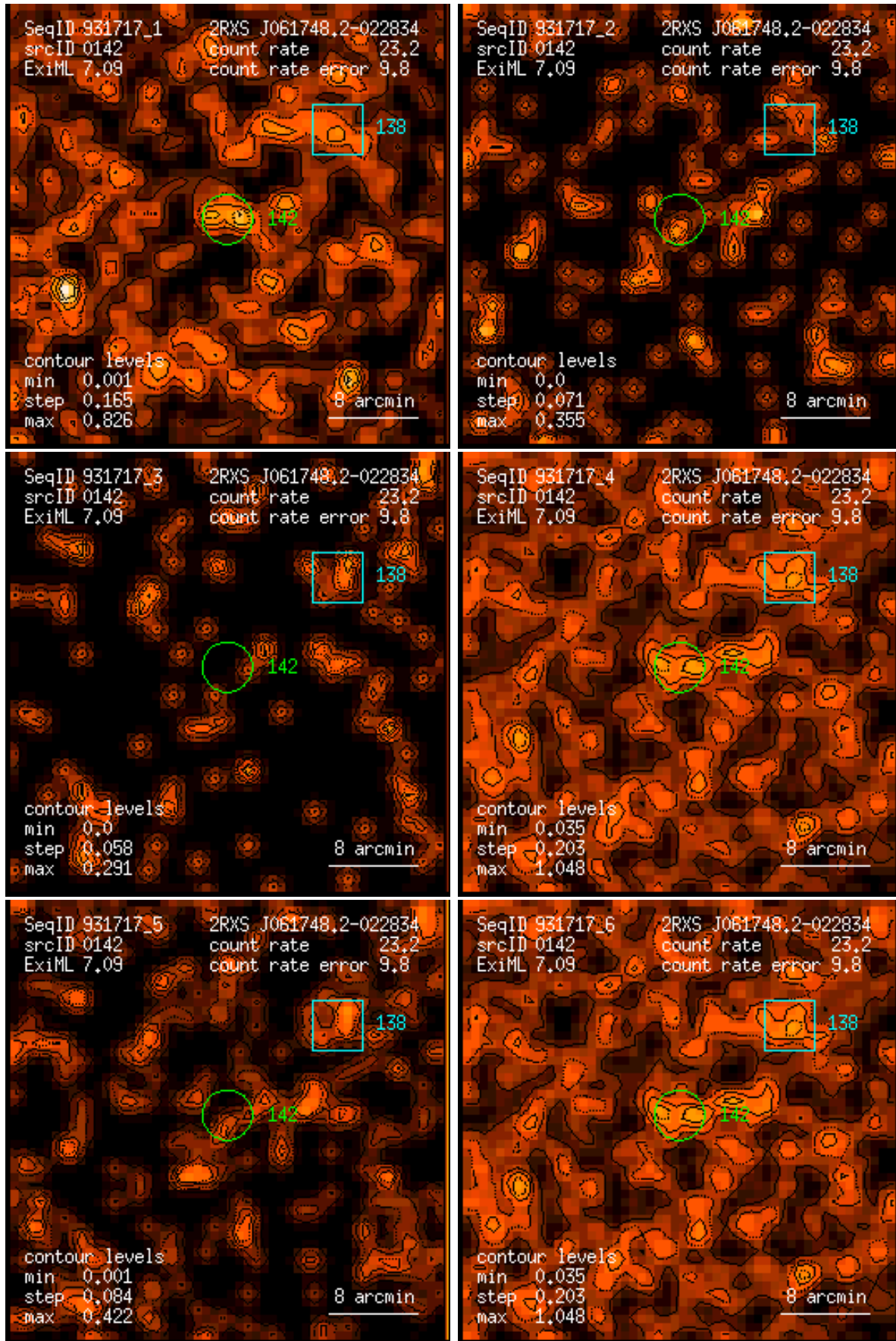
Figure 142: RASS 931717: detection 0142: band rate images, Gaussian filter: (1) PSPC channels 11 – 41, (2) 52 – 90, (3) 91 – 201, (4) 11 – 235, (5) 52 – 201, (6) 11 – 201. Broad band rates in counts/ks. Band rate contour levels in counts/ks/arcmin 2 .
