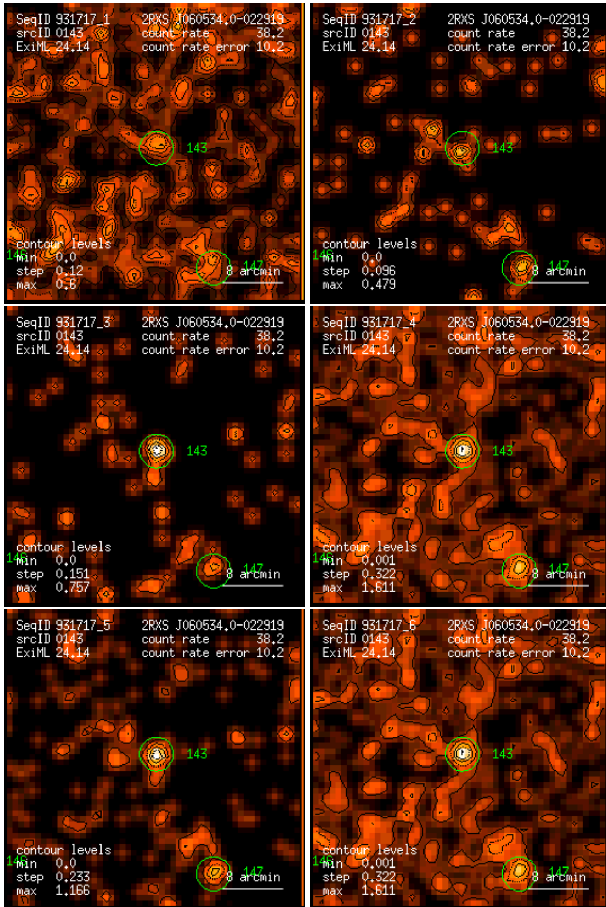
Figure 143: RASS 931717: detection 0143: band rate images, Gaussian filter: (1) PSPC channels 11 – 41, (2) 52 – 90, (3) 91 – 201, (4) 11 – 235, (5) 52 – 201, (6) 11 – 201. Broad band rates in counts/ks. Band rate contour levels in counts/ks/arcmin 2 .
