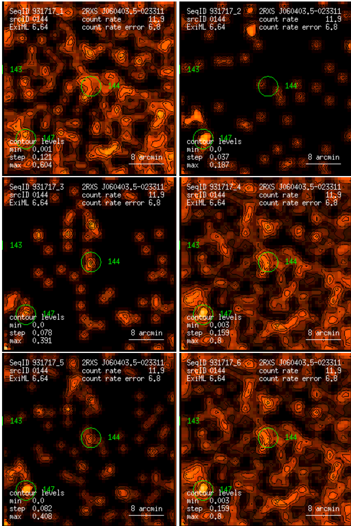
Figure 144: RASS 931717: detection 0144: band rate images, Gaussian filter: (1) PSPC channels 11 – 41, (2) 52 – 90, (3) 91 – 201, (4) 11 – 235, (5) 52 – 201, (6) 11 – 201. Broad band rates in counts/ks. Band rate contour levels in counts/ks/arcmin 2 .
