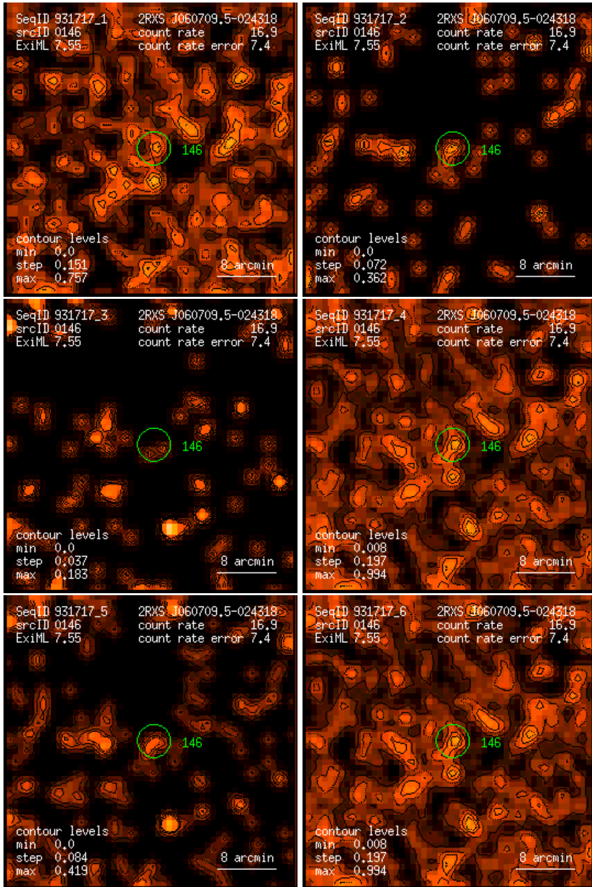
Figure 146: RASS 931717: detection 0146: band rate images, Gaussian filter: (1) PSPC channels 11 – 41, (2) 52 – 90, (3) 91 – 201, (4) 11 – 235, (5) 52 – 201, (6) 11 – 201. Broad band rates in counts/ks. Band rate contour levels in counts/ks/arcmin 2 .
