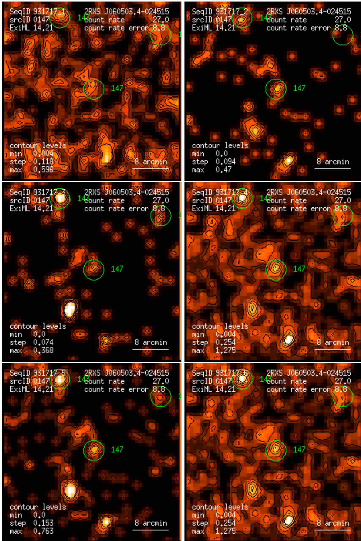
Figure 147: RASS 931717: detection 0147: band rate images, Gaussian filter: (1) PSPC channels 11 – 41, (2) 52 – 90, (3) 91 – 201, (4) 11 – 235, (5) 52 – 201, (6) 11 – 201. Broad band rates in counts/ks. Band rate contour levels in counts/ks/arcmin 2 .
